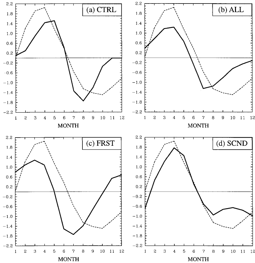
FIG. 4. Annual variations of SST averaged over the equatorial cold tongue obtained from (a) CTRL and the (b) all-year, (c) first-half-year, and (d) second-half-year experiments. The thin dashed curves in all panels are the annual variations from the observation.
