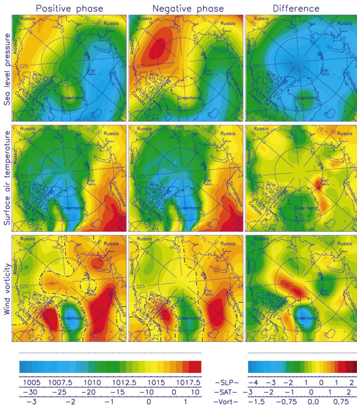
FIG. 5. (top) NCAR SLP (mb), (middle) NCEP–NCAR SAT (°C), and (bottom) wind vorticity (mb) computed from the NCAR SLP. The left (center) panels show the averages for the positive (negative) phases of the LFO, and the right panels show the difference between the positive and the negative phase.
