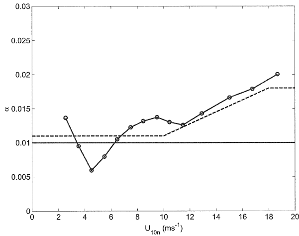
FIG. 11. Charnock parameter as a function of 10-m neutral wind using the mean turbulence values (O) from Fig. 10. The dashed line is COARE 3.0; the solid straight line a value of 0.01.
