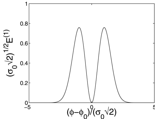
FIG. 4. Leading EOF of pure Gaussian fluctuations in jet width [Eq. (39)]. Normalization as in Fig. 2.
