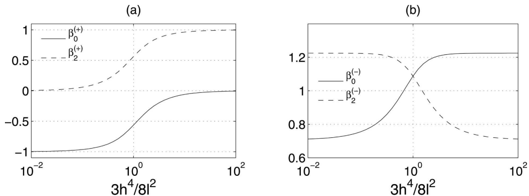
FIG. 6. Components of the EOFs spanned by f_0(\phi) and f_2(\phi) for fluctuations in both jet strength and position, for (a) the EOF with the larger variance \mu^{(+)} and (b) the EOF with the smaller variance \mu^{(-)} .
