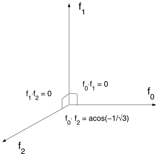
FIG. 3. Geometric illustration of the vectors (in function space) f_0(\phi) , f_1(\phi) , and f_2(\phi) . Because f_0(\phi) and f_2(\phi) are not orthogonal, they cannot simultaneously be eigenvectors of a symmetric function such as the covariance. If both of these vectors contribute to the leading EOFs, these EOFs must be orthogonal linear combinations of these vectors.
