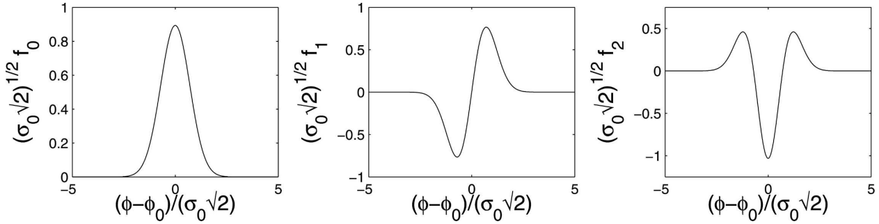
FIG. 2. Plots of the functions f_0(\phi) , f_1(\phi) , and f_2(\phi) [Eqs. (11)–(13)] from which the leading EOFs are constructed, rescaled to be of unit norm.
