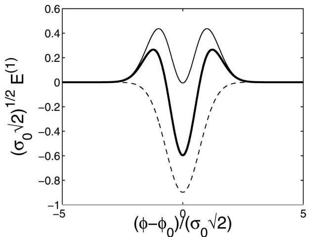
FIG. 9. Leading EOF in case of correlated strength and inverse width fluctuations, for \rho/U_0 = 0.01 (thin solid line), \rho/U_0 = 1 (thick solid line), and \rho/U_0 = 100 (dashed line).
