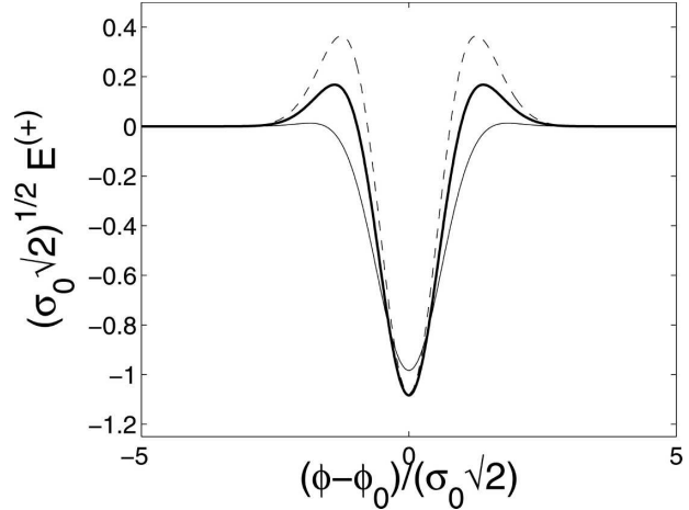
FIG. 7. Hybrid EOFs E^{(+)} of the covariance function (44) for values of the ratio 3h^4/8l^2 equal to 0.3 (thin solid curve), 1 (thick curve), and 3 (dashed curve).
