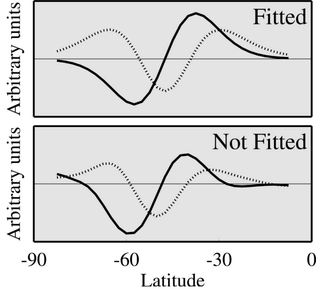
FIG. 1. Leading EOFs of daily Southern Hemisphere winter (May–September) 500-hPa zonal mean zonal wind (1958–2003). (top) Following the fitting procedure in accord with Eqs. (1)–(7). (bottom) Not following the fitting procedure. Solid curves: E^{(1)} . Dashed curves: E^{(2)} .
