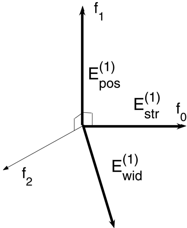
FIG. 5. The orientations in the space spanned by f_0(\phi) , f_1(\phi) , and f_2(\phi) of the leading EOFs for the cases of pure fluctuations in jet strength, position, and width.
