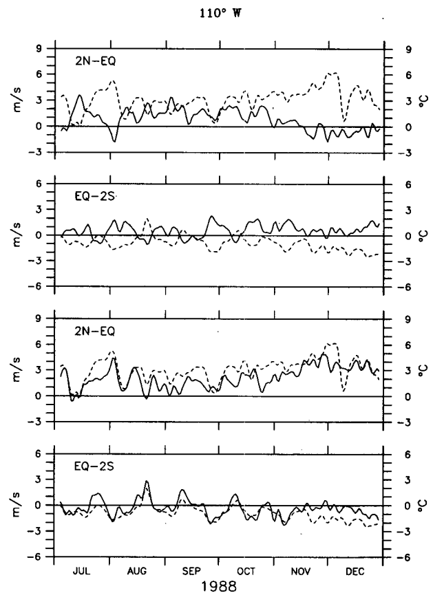
FIG. 6. Low-pass filtered time series during the period July through December 1988. Top two panels are the differences in zonal wind (solid) and SST (dashed) between 2^{\circ}\text{N} and the equator and between the equator and 2^{\circ}\text{S} ; bottom two panels are the differences in scalar wind speed (solid) and SST (dashed) over the same latitudes.
