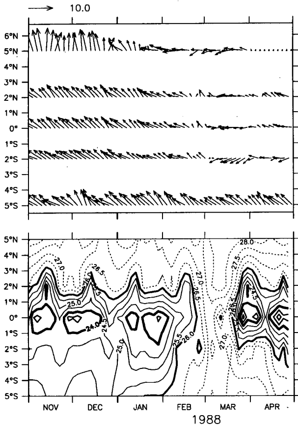
FIG. 2. Wind vectors and SST contours along 110°W based on the moored measurements at 5°N, 2°N, 0°, 2°S, and 5°S from November 1987 through April 1988. Time series were filtered with a 5-day Hanning filter prior to plotting. Wind and SST measurements at 5°N stopped on 30 March; after that time 20 m temperature was used in place of SST in the contour plot. Temperature contour interval is 0.5°C. Arrow at top of figure indicates scale of wind vectors in meters per second.
