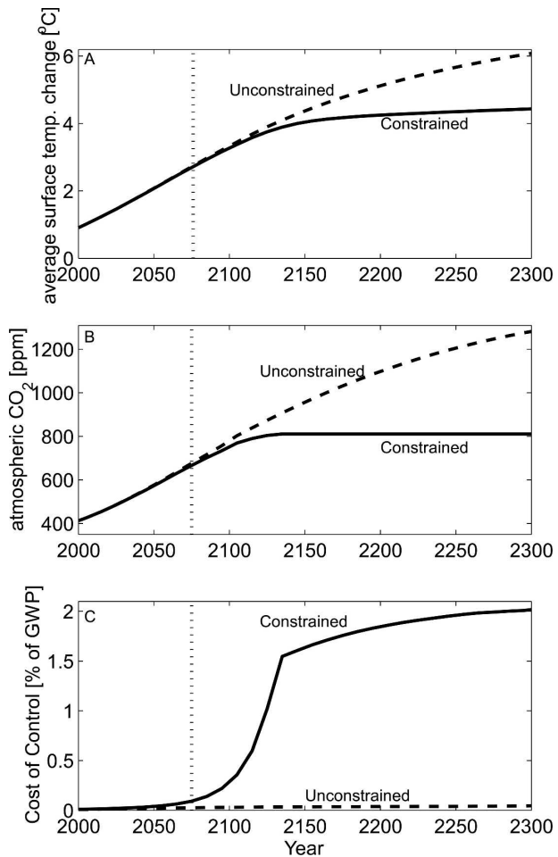
FIG. 4. Estimation of the additional costs of avoiding an MOC collapse. The calculations are based on the DICE-94 model of Nordhaus (1994) with the additional constraint to keep the equivalent \text{CO}_2 concentrations below the critical level to preserve the MOC in the model of Stocker and Schmittner (1997). (a) The effects of the (b) reduced atmospheric \text{CO}_2 concentrations on globally averaged surface temperatures are shown. (c) The dashed vertical line illustrates the time when the investments in \text{CO}_2 abatement start to diverge considerably. This time is the adopted decision point in this specific example.
