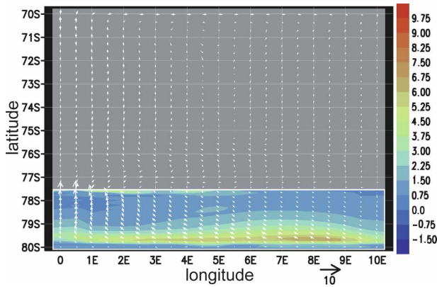
FIG. 6. Basal melt rate ( \text{m yr}^{-1} ) overlain by mixed layer velocity vectors ( \text{cm s}^{-1} , plotted every grid point in longitude and every second grid point in latitude) in simulation D_{+1.0} . Scales are chosen to be the same as in Fig. 4c for comparative purposes. Gray shading indicates the absence of the ice shelf.
