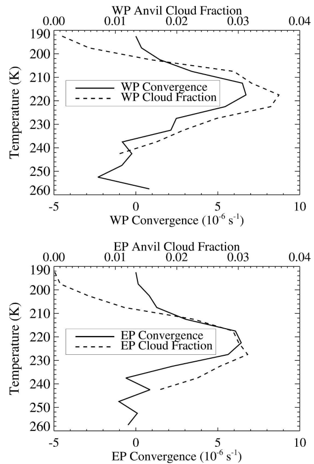
FIG. 13. Clear-sky convergence and anvil cloud fraction for (top) WP and (bottom) EP for September 2004–July 2005.
