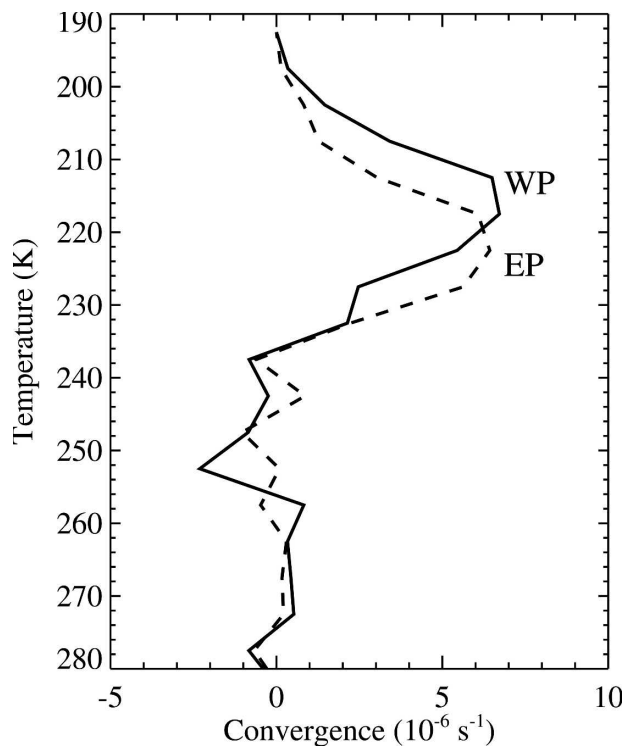
FIG. 12. Binned clear-sky convergence profiles for WP and EP for September 2004–July 2005.
