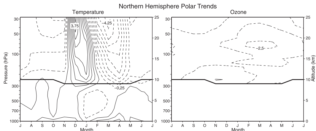
FIG. 2. As in Fig. 1, but for (left) 60^{\circ} – 90^{\circ} N and (right) 65^{\circ} – 90^{\circ} N. The lower bound for Fig. 2 is 1000 hPa.
