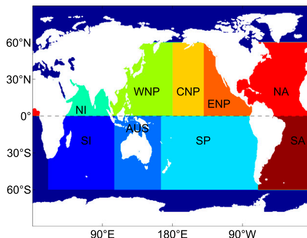
FIG. 1. Our basin definitions and abbreviations used in subsequent figures.
