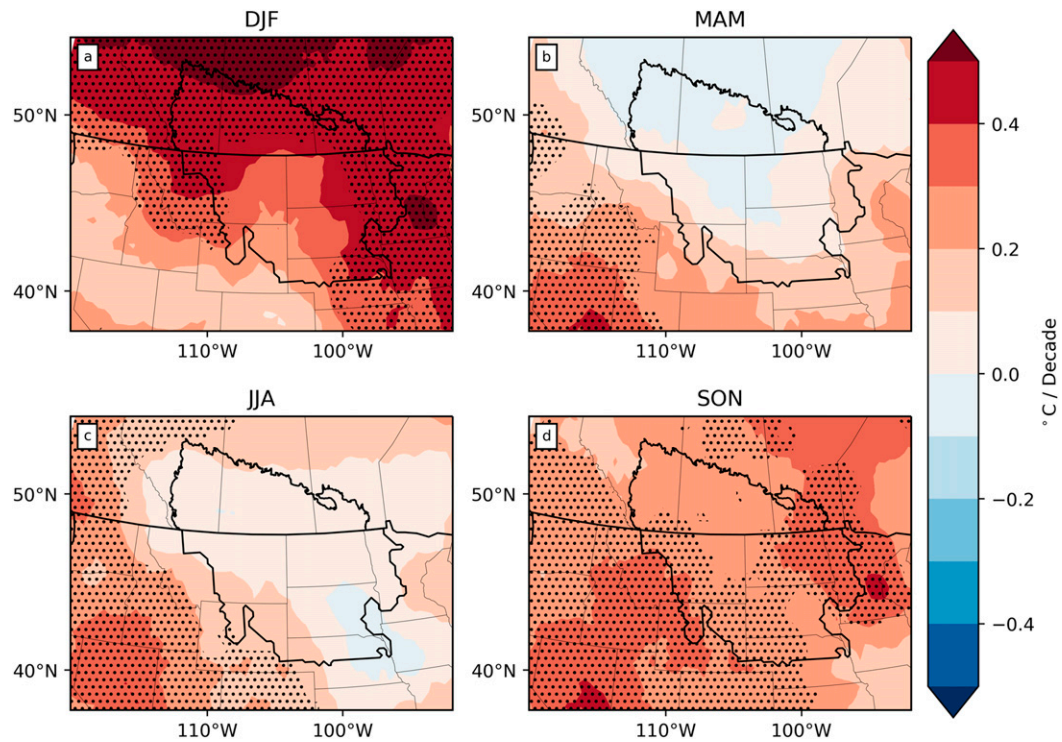
FIG. 2. Trends in 2-m air temperature T_{\text{air}} from 1970 to 2015 across the NNAGP and surrounding regions. Stippling indicates a significant trend at p < 0.05 after correcting for autocorrelation [Eq. (1)] against a null hypothesis of no trend.
