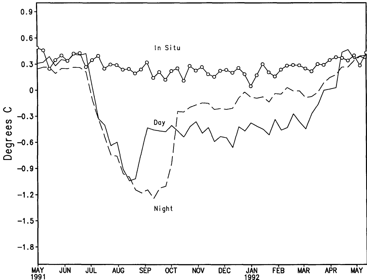
FIG. 3. Time series of the in situ, daytime, and nighttime satellite SST anomalies (see text) between 20^{\circ}\text{N} and 20^{\circ}\text{S} for 55 weeks. The in situ curve is a solid line with circles, the daytime curve is a solid line, the nighttime curve is dashed. The abscissa is as given in Fig. 2. The ordinate is in degrees Celsius.
