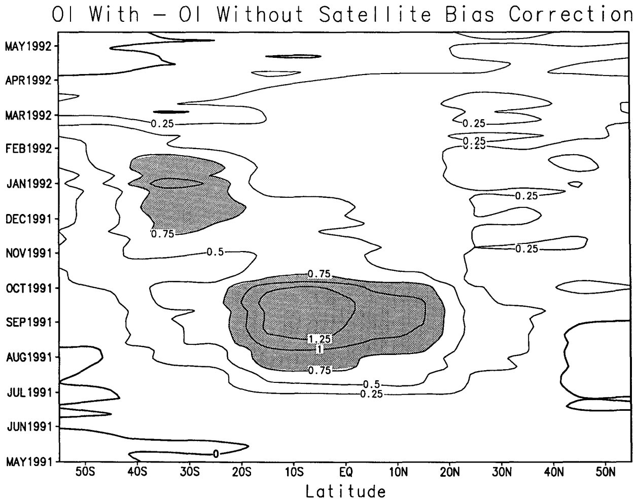
FIG. 5. Zonally averaged difference between the OI with and without the satellite bias correction for the 55-week period defined in Fig. 2. The sign of the difference is with - without satellite correction. Otherwise as in Fig. 4.
