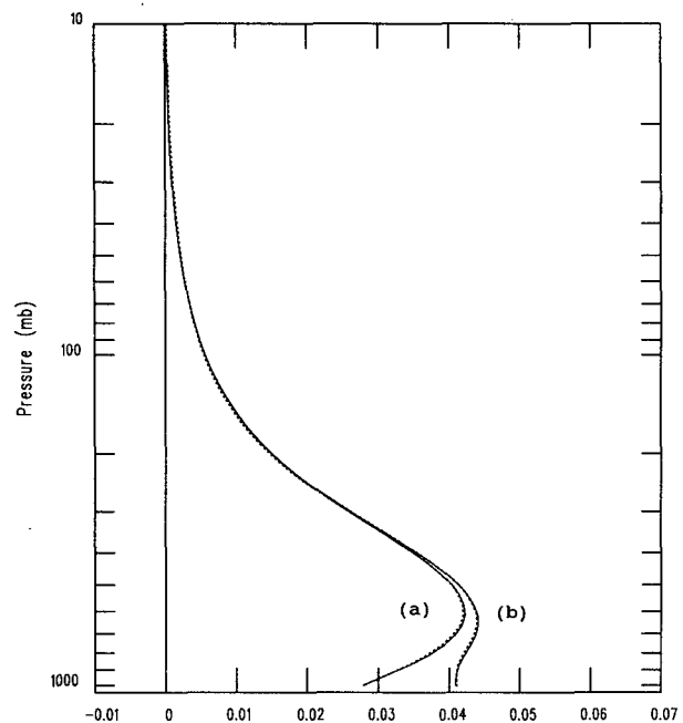
FIG. 10. Actual and AMSU-derived MSU channel 2 weighting functions for surface emissivities of (a) 1.0 and (b) 0.5.
