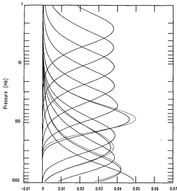
FIG. 9. Comparison of AMSU and MSU (dotted curves) weighting functions.
