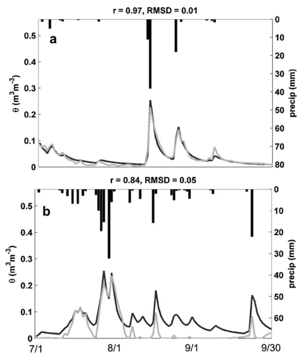
FIG. 3. Daily precipitation (bars), in situ soil moisture (gray), and modeled soil moisture at a collocated gauge (black) for a (a) “good” fit (gauge 100; 2009) and (b) “poor” fit (gauge 34; 2010) from 1 Jul to 30 Sep. Correlation and RMSD of modeled to in situ soil moisture are labeled.
