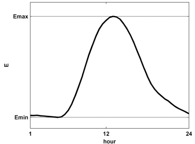
FIG. 2. The diurnal cycle of max surface evapotranspiration E ( \text{mm h}^{-1} ) in Eq. (1) as a function of local hour, as estimated from flux measurements at the Kendall site in WGEW. The variable E_{\text{min}} is approximately 1/10 of E_{\text{max}} , and E_{\text{max}} is provided in Table 1.
