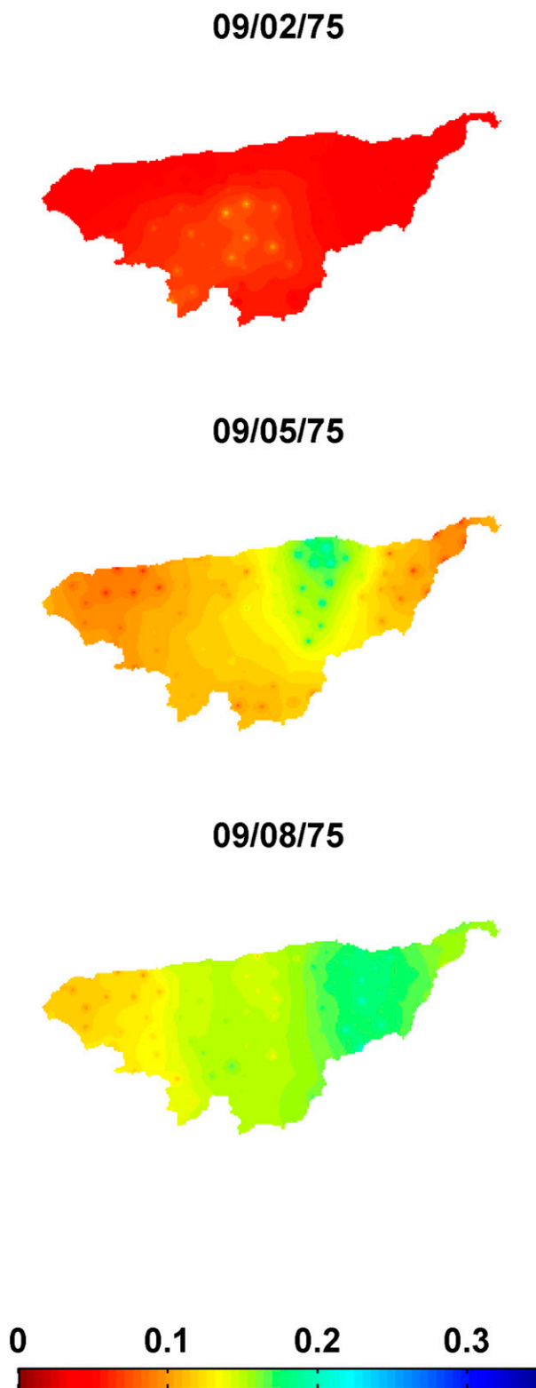
FIG. 5. Spatial distribution of daily avg soil moisture ( \text{m}^3 \text{m}^{-3} ) for 2, 5, and 8 Sep 1975 over WGEW centered at 31°43'N, 110°41'W.
