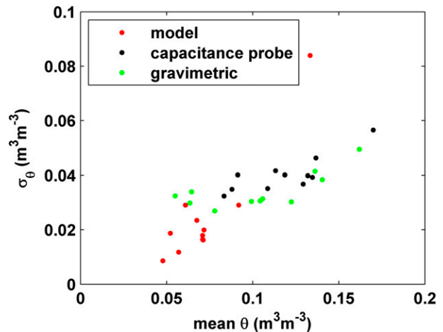
FIG. 8. Spatial std dev of 800-m, 30-min gridded modeled (red), in situ capacitance probe (black), and gravimetric (green) soil moisture as a function of spatially averaged soil moisture for the 11 days during which gravimetric sampling was done during SMEX04.
