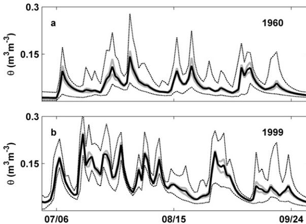
FIG. 6. Spatially averaged (over all 100\text{ m} \times 100\text{ m} grid cells) daily soil moisture (solid black), 25th and 75th percentile soil moisture values (gray), and min and max soil moisture values (dotted black) within WGEW for (a) 1960 and (b) 1999.
