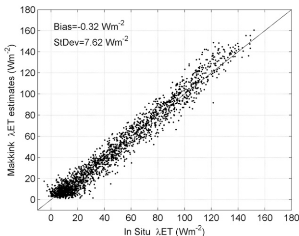
FIG. 8. Test of the revised Makkink Eq. (7) as proposed by de Bruin (1987) . Daily values are for Cabauw during 2007–12.
