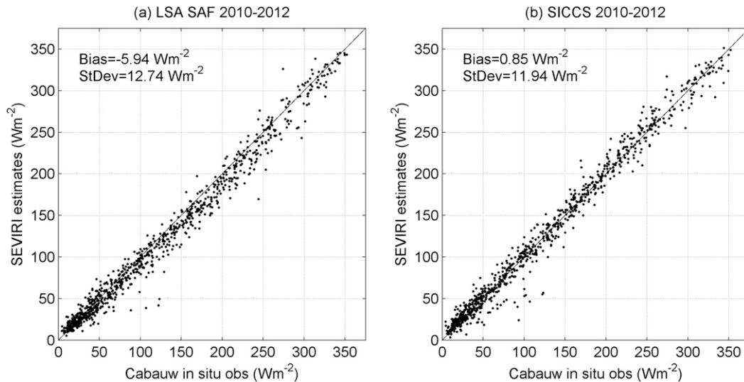
FIG. 4. Scatterplots of daily solar radiation estimates from SEVIRI MSG ( \text{W m}^{-2} ) against in situ observations in Cabauw considering (a) LSA SAF and (b) SICCS products. The mean (bias) and standard deviation of differences are also displayed.
