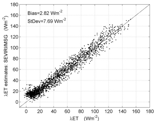
FIG. 6. As in Fig. 2, but for SEVIRI MSG global radiation (SICCS) as input.
