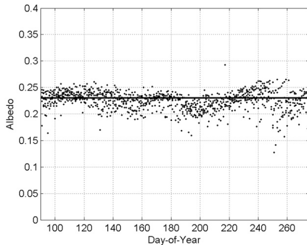
FIG. 1. Measured albedo for days of the year 90–275 at Cabauw during 2007–12.
