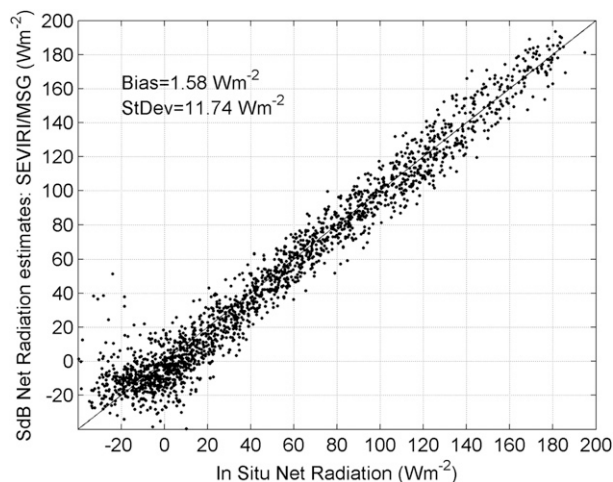
FIG. 5. As in Fig. 3, but for SEVIRI MSG global radiation according the SICCS algorithm.
