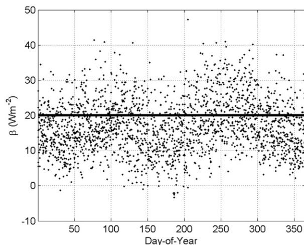
FIG. 7. Measured \beta as function of day of year.
