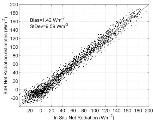
FIG. 3. Test net radiation formula of SdB at Cabauw during 2007–12.
