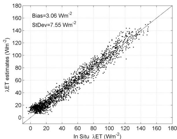
FIG. 2. Latent heat flux estimated according to Eq. (6), that is, using the SdB net radiation formula, plotted against in situ measured values: daily values at Cabauw during 2007–12 except for a limited number of dry and advective days (see text).
