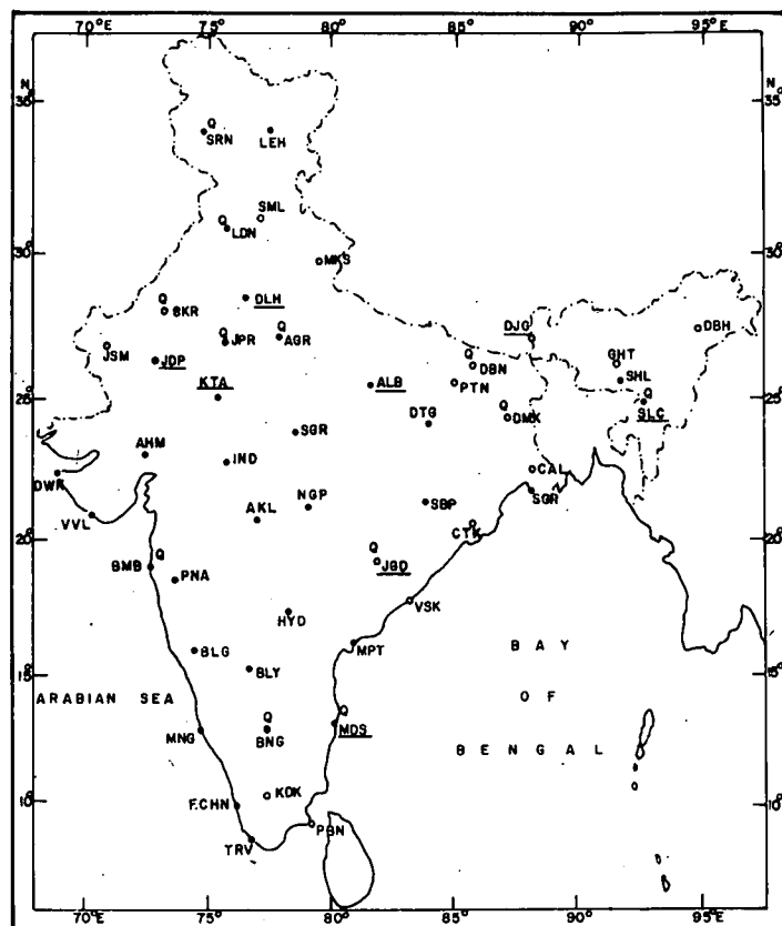
FIGURE 2.—Observing stations from which rainfall data were used. Here, (●) indicates increasing trend, (○) indicates decreasing trend, Q indicates QBO, and underline indicates 11-yr cycle. (Note that all stations indicate either an increasing or decreasing trend; those with significant trends are named in section 3.)
