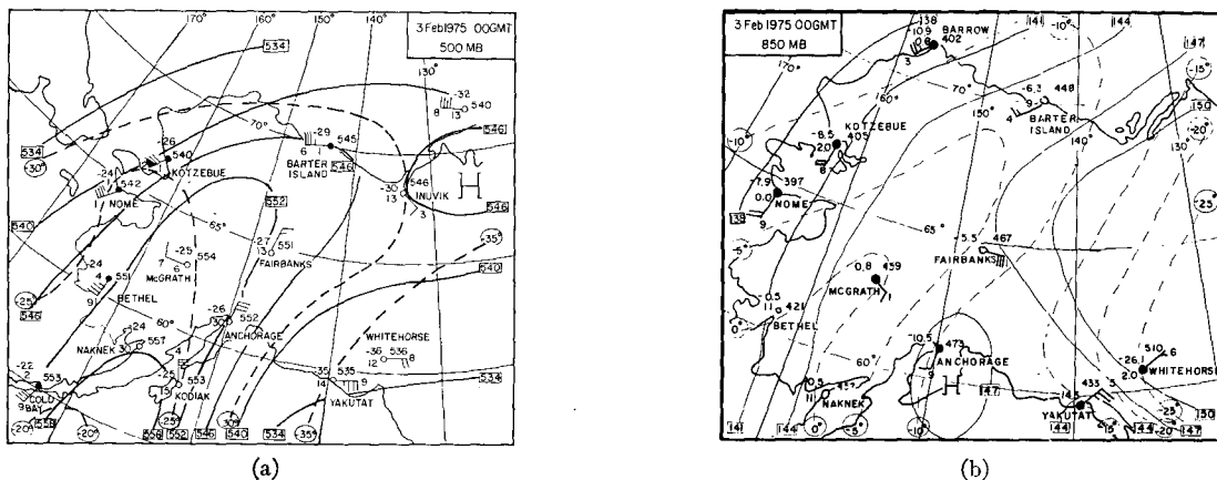
FIG. 5. Upper air pressure systems typical of these valley wind situations: (a) 500 mb, (b) 850 mb.
