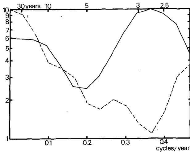
FIG. 1. Normalized power spectra for the time series presented in Table 1 (Africa, full line; India, dashed line).
