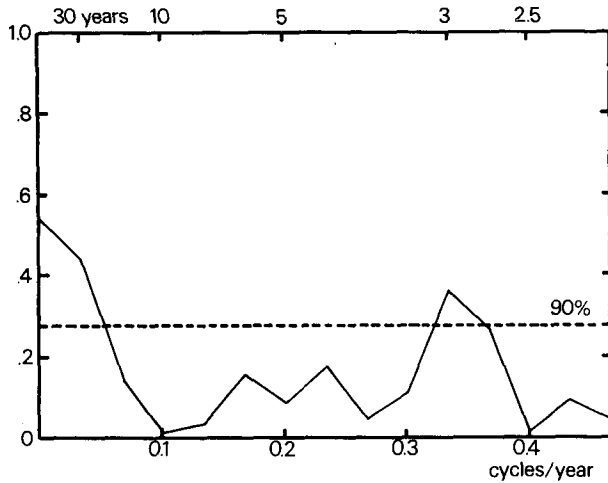
FIG. 2. Coherence of the two time series presented in Table 1. The dashed line represents the 90% significance level.
