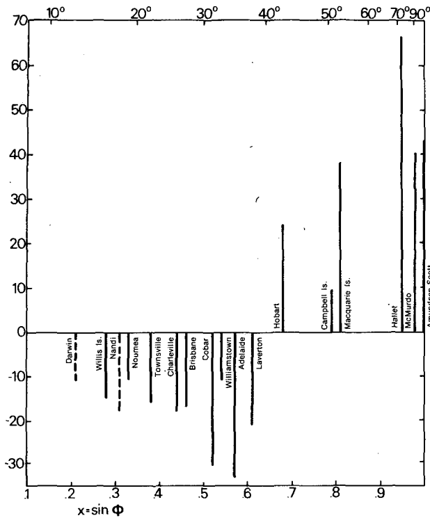
FIG. 5. 1972 anomalies (m) from station record mean of the mean annual 500 mb surface height. Data used for this cross section included all available stations within the longitude sector of 150°E±10° (with Darwin and Nandi also included although they are outside this sector).
