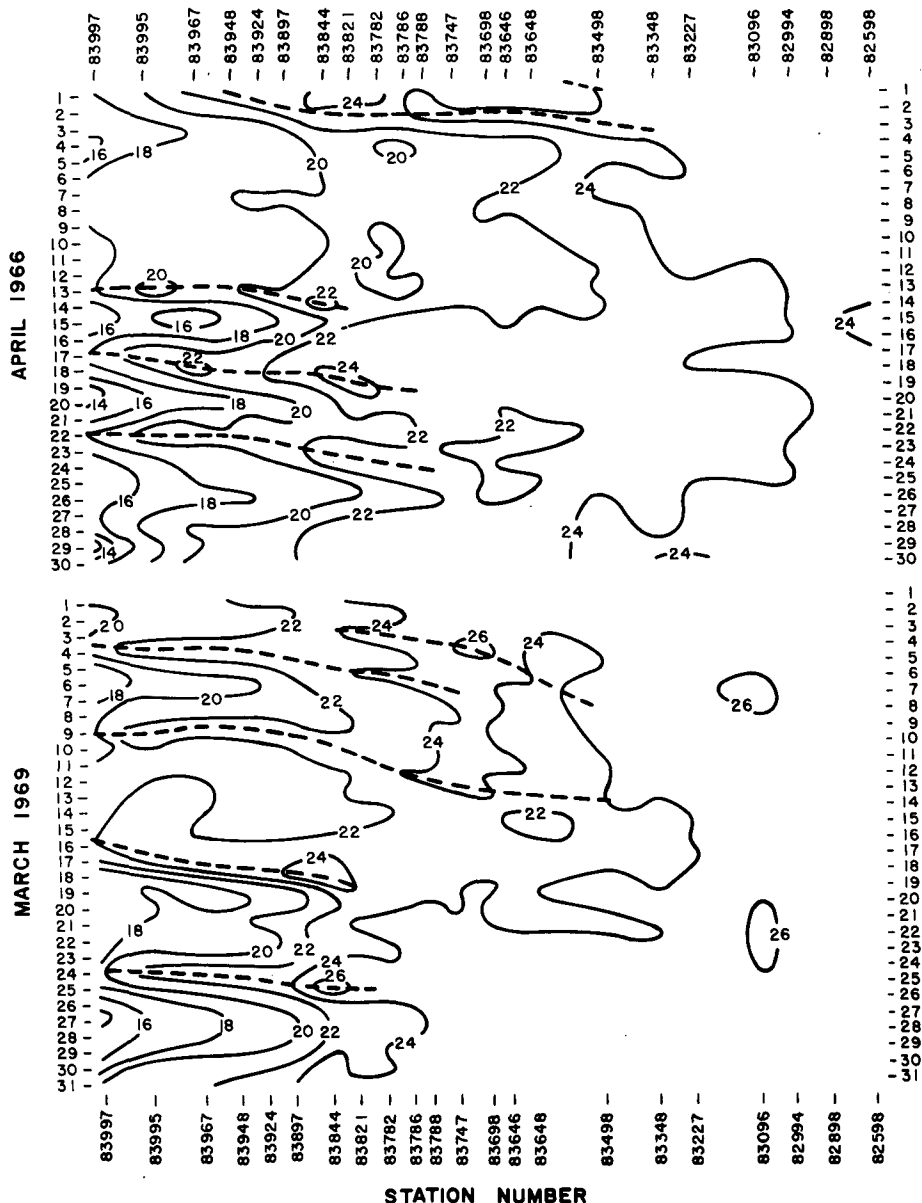
FIG. 12. As in Fig. 6 except for April 1966 and March 1969.
