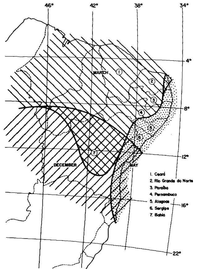
FIG. 3. Areal distribution of the month in which the mean monthly rainfall reaches a maximum. Data used are for the period 1931–1960 and were obtained from the Superintendência do Desenvolvimento do Nordeste in Recife, Pernambuco.
