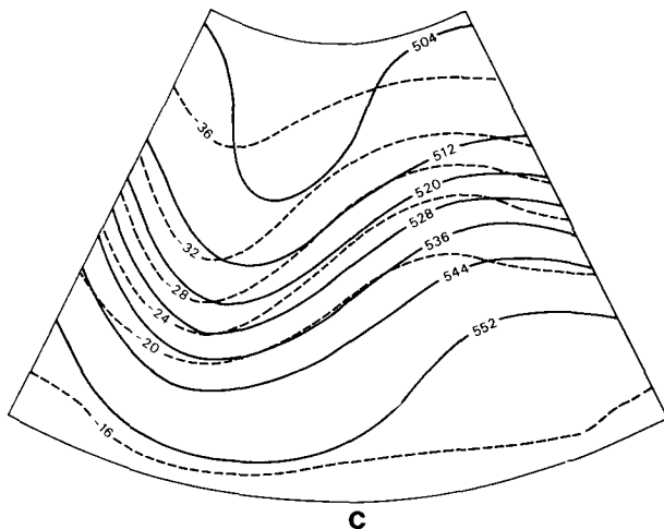
FIG. 1. Situation after 96 h of integration, when the mountain is inserted: (a) mean sea level (MSL) pressure (last two digits of the value in mb); (b) geopotential (dam) and temperature ( ^{\circ}\text{C} ) at 850 mb; (c) geopotential and temperature at 500 mb.
