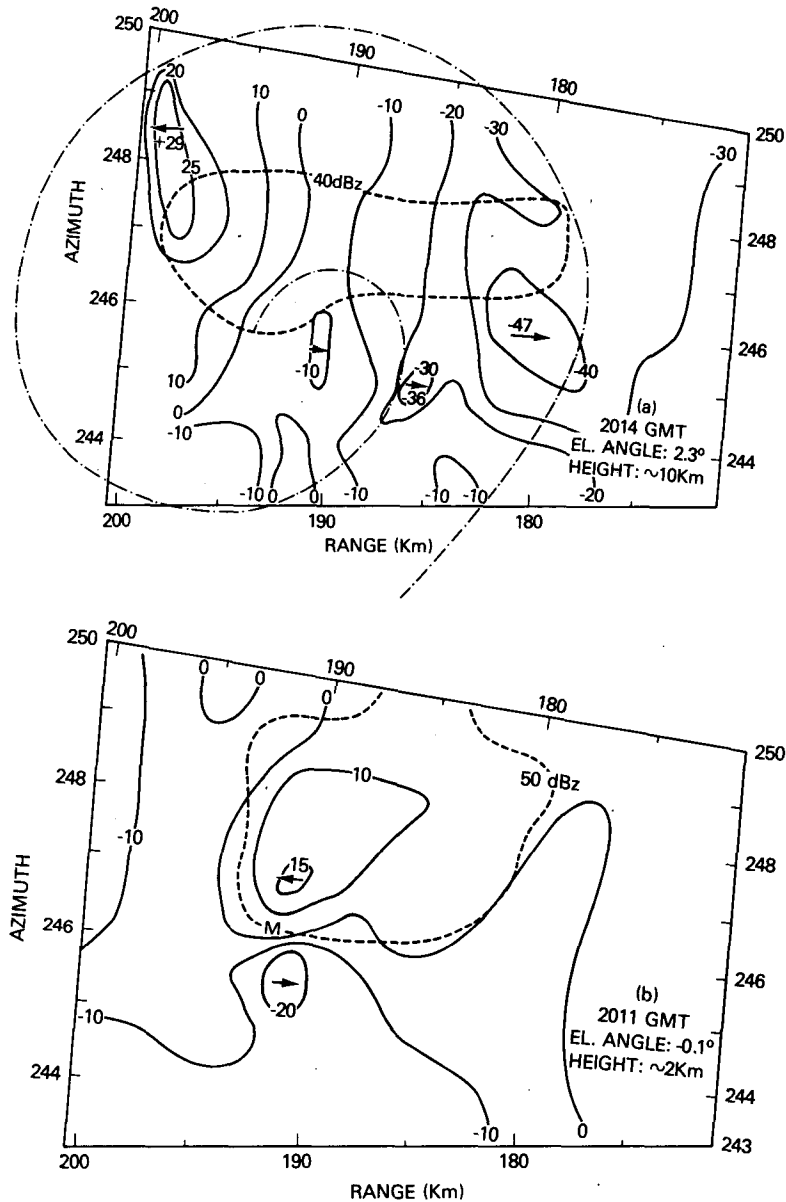
FIG. 3. Single Doppler radar radial velocities observed by National Severe Storms Laboratory radar at Norman, Oklahoma. Solid lines are velocities in meters per second, with positive values indicating flow away from the radar. A mean storm motion of 10 \text{ m s}^{-1} toward the radar has been subtracted from the original values. The dashed lines are reflectivity contours. (a) Flow pattern at 10 km at 2014 GMT 20 May 1977; dash-dot line is satellite-observed spiral feature at 2004 GMT. (b) Flow pattern at 2 km at 2011 GMT 20 May 1977; M indicates mesocyclone position at that altitude.
