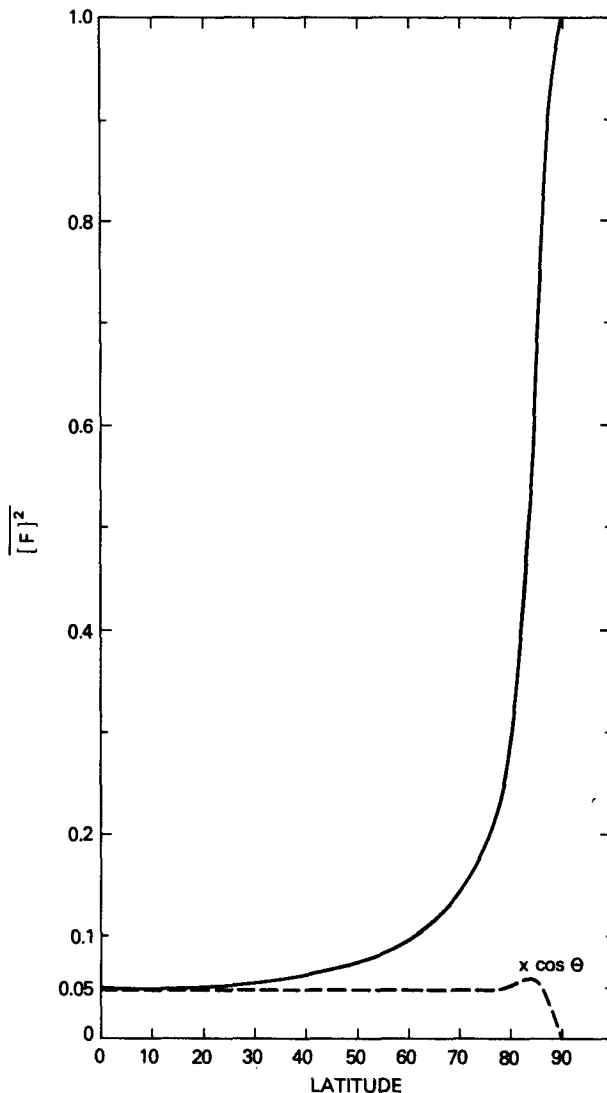
FIG. 2. The solid curve shows the variance of the zonal mean of the random field F computed from Eq. (6) using the spectrum plotted in Fig. 1. The dashed curve shows the solid curve multiplied by \cos\theta .
