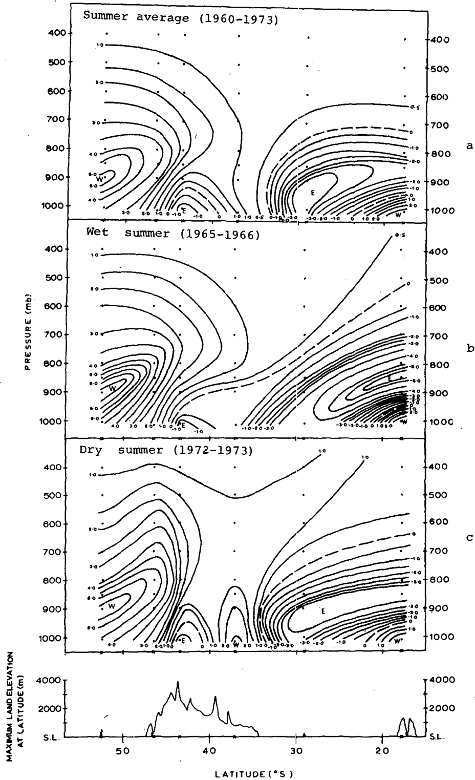
FIG. 6. Mean zonal transport of water vapor across 175°E for: (a) summer average (1960-73), (b) wet summer (1965-66) and (c) dry summer (1972-73). Units are 10^{-1} \text{ kg m}^{-1} \text{ mb}^{-1} \text{ s}^{-1} .
