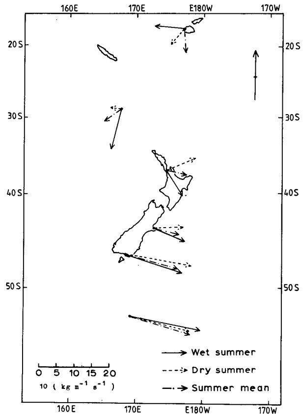
FIG. 12. Mean vertically integrated vector transport of water vapor for: summer average (1960-73); wet summer (1965-66), and dry summer (1972-73). Units are 10 kg m -1 s -1 .
