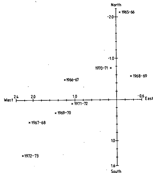
FIG. 14. Vector diagram of the mean of the surface and 900 mb zonal and meridional water vapor transfer over Auckland for each summer from 1965 to 1973. Vector is obtained by drawing the line from the cross to the origin. Units are 10^{-1} \text{ kg m}^{-1} \text{ mb}^{-1} \text{ s}^{-1} .
