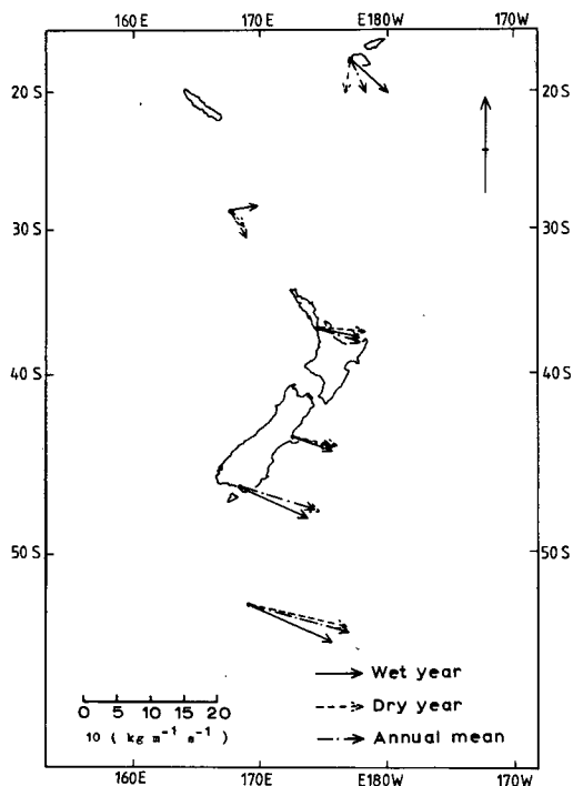
FIG. 11. Mean vertically integrated vector transport of water vapor: annual average (1960-73); wet year (1968) and dry year (1973). Units are 10 kg m -1 s -1 .
