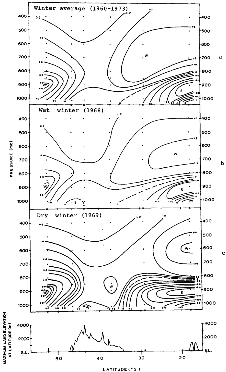
FIG. 7. Mean zonal transport of water vapor across 175°E for: (a) winter average (1960-73), (b) wet winter (1968), and (c) dry winter (1969). Units are 10^{-1} \text{ kg m}^{-1} \text{ mb}^{-1} \text{ s}^{-1} .
