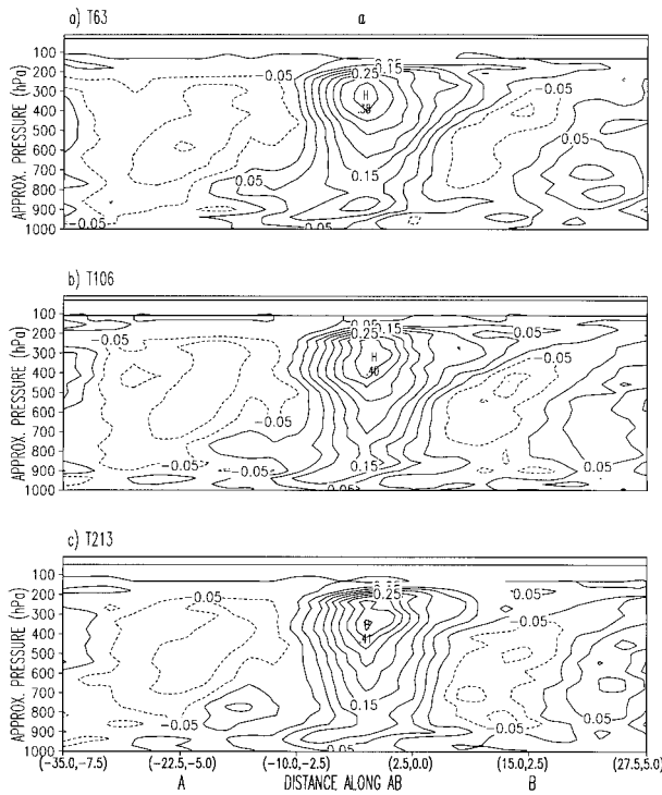
FIG. 5. As in Fig. 4 but for cloud fraction (interval: 0.05, dimensionless).
