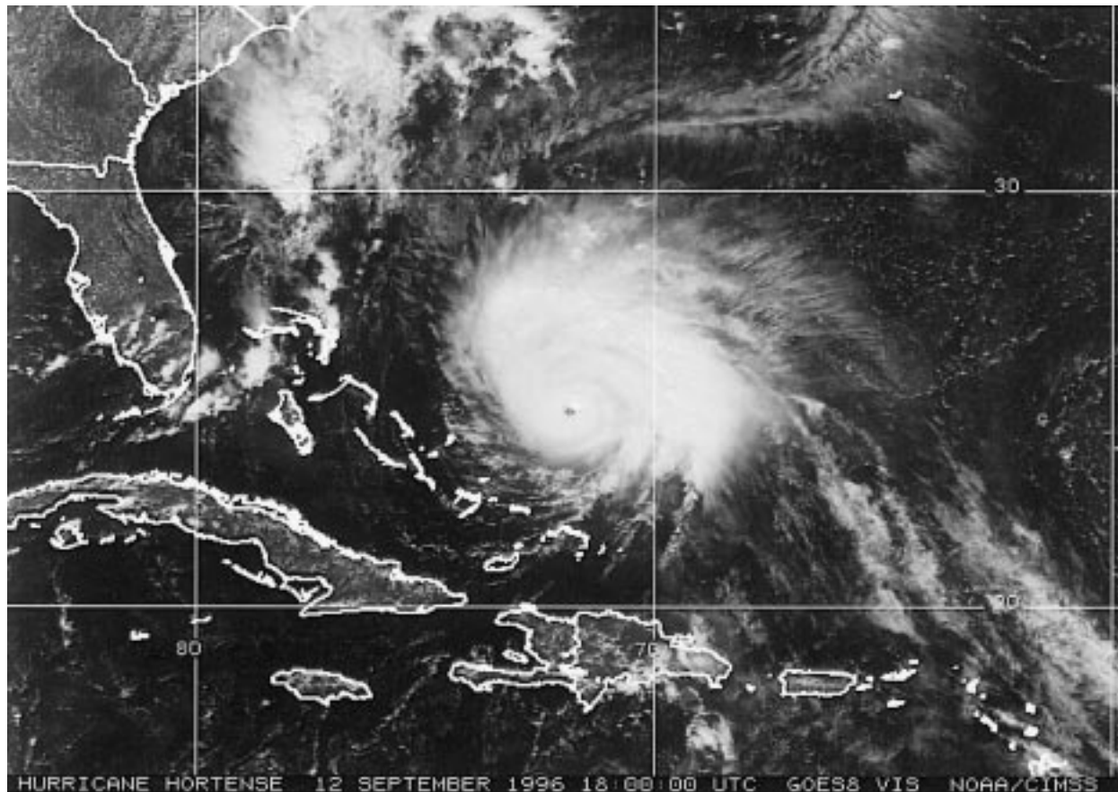
FIG. 9. Visible GOES-8 satellite image of Hurricane Hortense at 1800 UTC 12 September 1996, just before peak intensity. Note the well-defined eye.
