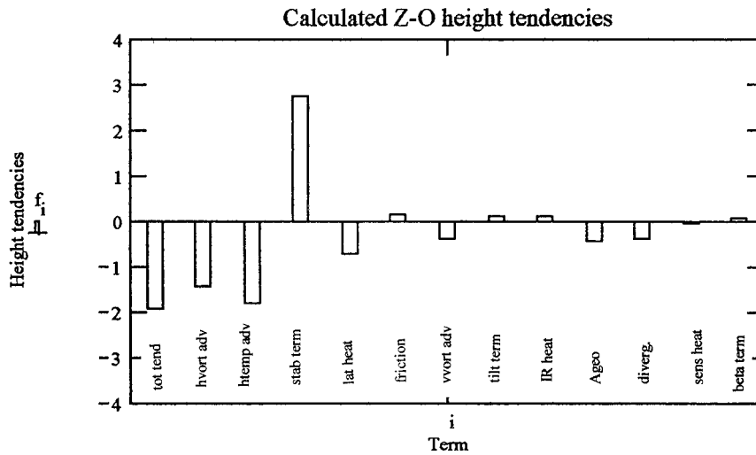
FIG. 2. Bar graph displaying averaged center point Z-O calculated height tendencies ( \times 10^{-3} m s -1 ) for the cyclone over eastern Kansas and Nebraska (37.5°N, 97.5°W) at 0000 UTC 10 Nov 1998.
