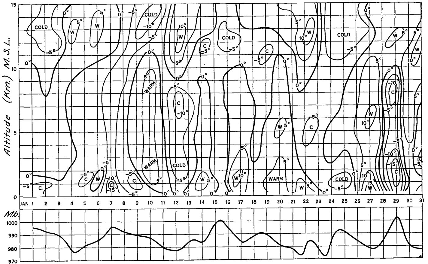
FIGURE 4.—The lines at the top connect points of equal departure (°C.) from the average temperature for the month, and the curve at the bottom shows the surface pressure plotted against day of the month.
