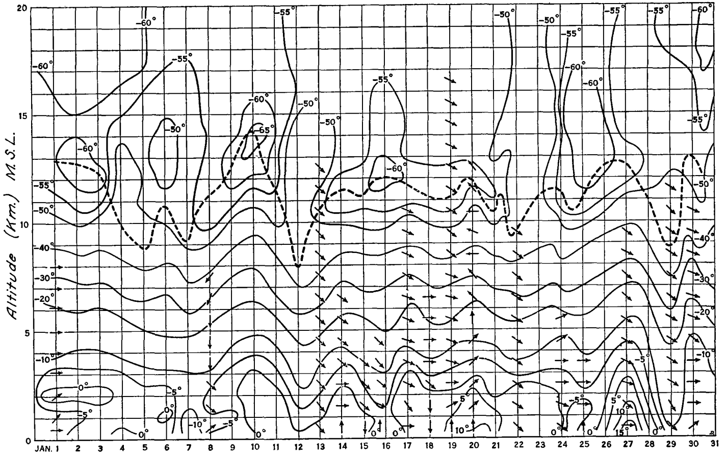
FIGURE 3.—Free-air isotherms (solid lines), height of the tropopause (heavy dashed line), and wind directions (arrows) for January 1934 at Omaha, Nebr.
