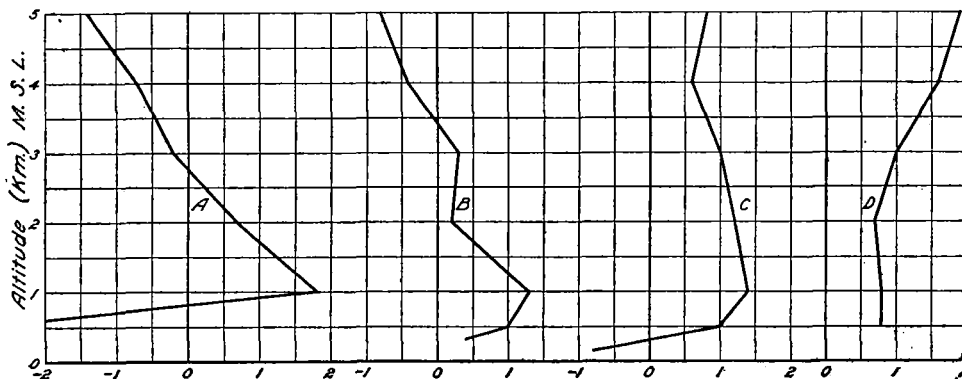
FIGURE 2.—Average difference (°C.), temperature observed by airplanes minus temperature observed by sounding-balloon, (a) at Omaha, Nebr., during January 1934, (b) at Omaha, Nebr., during Polar Year, (c) at Dallas, Tex. during Polar Year; and (d) average difference (°C.) temperature observed by old-type aerometeorograph minus temperature observed by new-type aerometeorograph.
