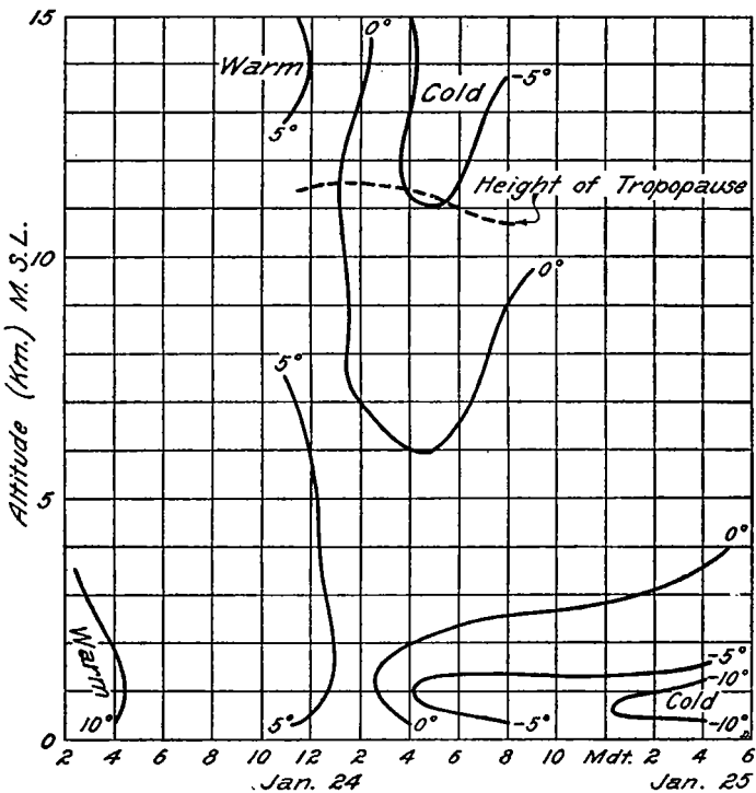
FIGURE 6.—Lines of equal departure (°C.) on the 24th and 25th from the average temperature for the month.
