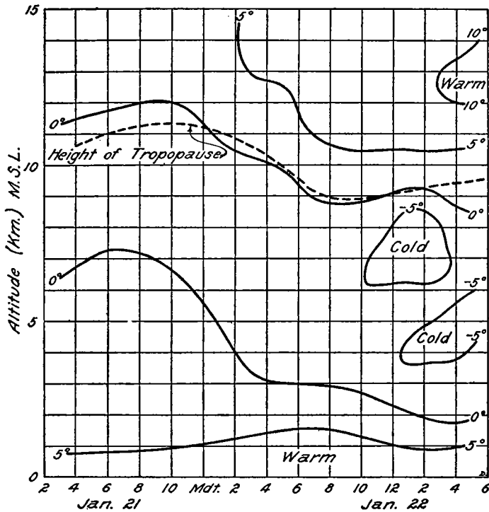
FIGURE 5.—Lines of equal departure (°C.) on the 21st and 22d from the average temperature for the month.
