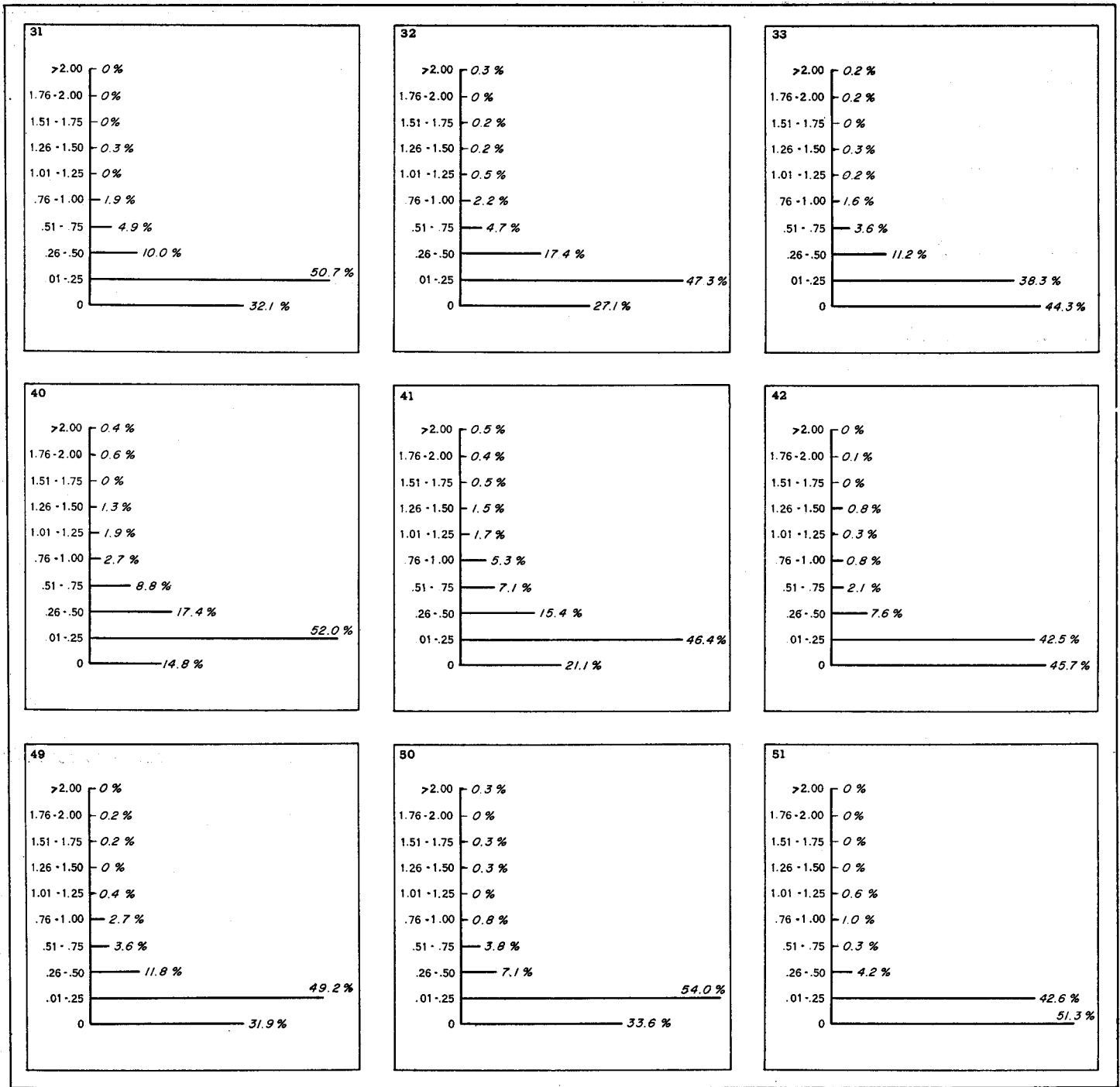
FIGURE 5.—Frequency distribution of hourly rainfall amounts around the center of the hurricane. See figure 3 for the location of the squares by number.
