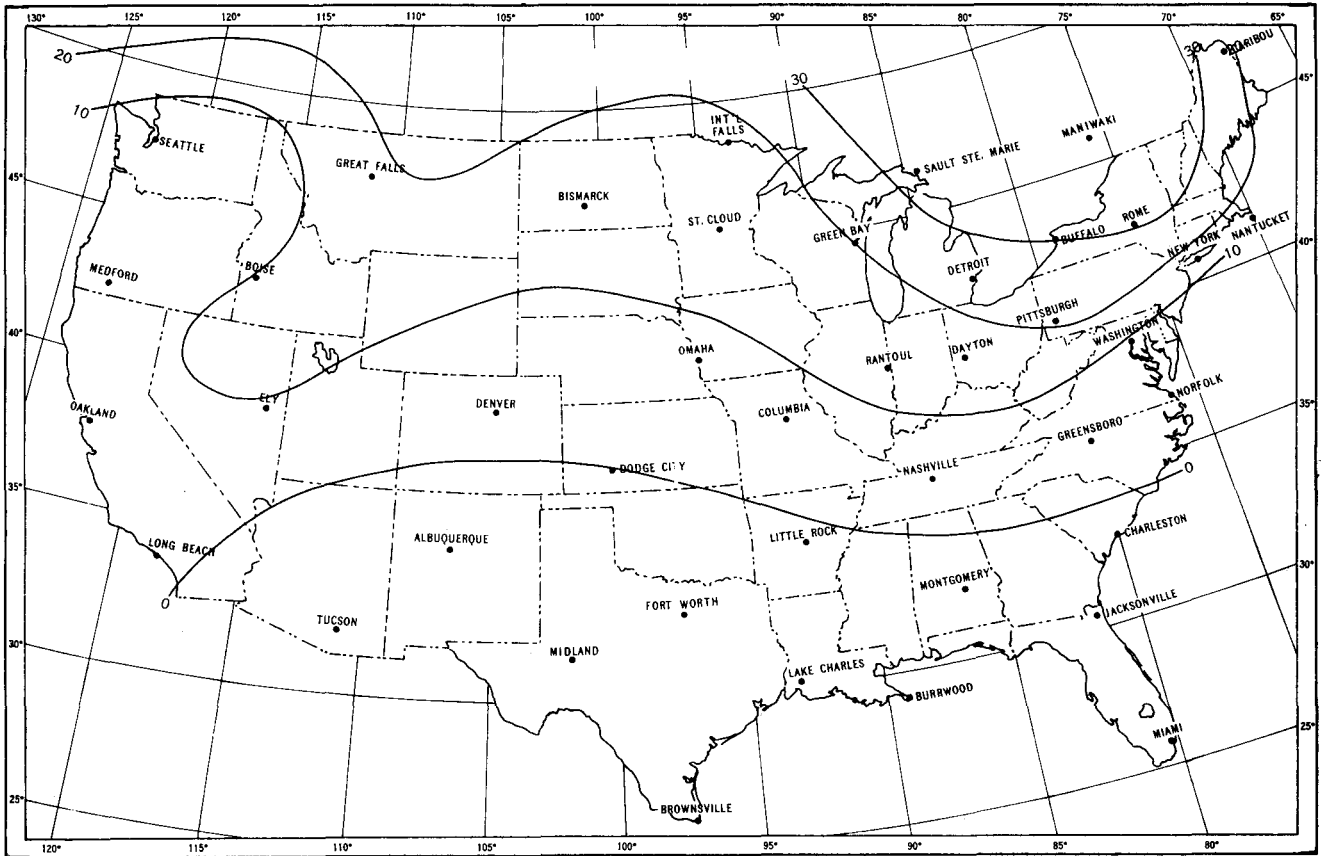
FIGURE 2.—Percentage of soundings with winds \geq 100 m.p.h. July 1957-58.
