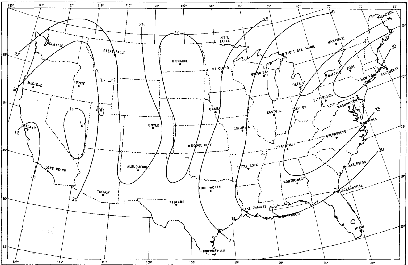
FIGURE 3.—Percentage of soundings with winds \geq 100 m.p.h. All months 1957-58.
