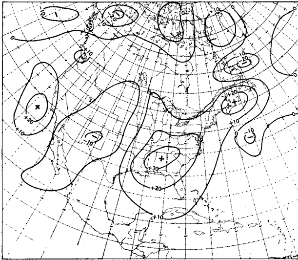
FIGURE 7.—Error in decafect of 12-hr. barotropic forecast from 0000 GMT December 6, 1959.
