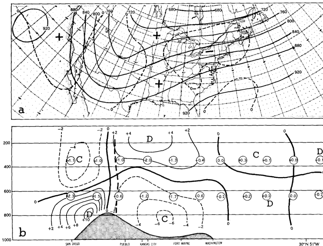
FIGURE 2.—(a) Error in decafeet (dashed lines) of the 12-hr. barotropic forecast from 0000 GMT, January 21, 1959, superimposed on the 500-mb. contours (solid lines) for that time. (b) Cross-section of horizontal divergence in units of 10^{-6} \text{ sec.}^{-1} . The numbers in circles are \omega in units of 10^{-3} \text{ mb. sec.}^{-1} . Heavy dashed line is the trough line.
