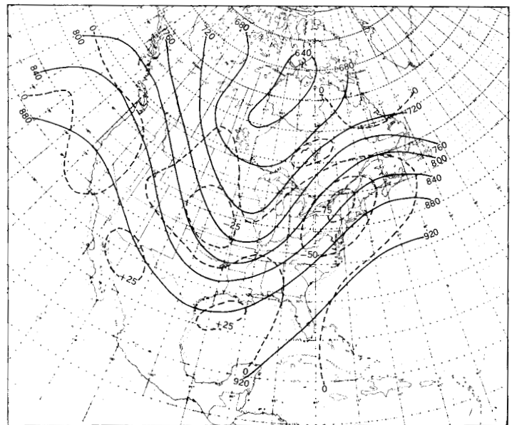
FIGURE 5.—Contribution of the vertical advection of momentum to the 500-mb. height tendency (dashed lines; units of ft. per 12 hr.) for 0000 GMT January 22, 1959, superimposed on the 500-mb. contours (solid lines) for that time.
