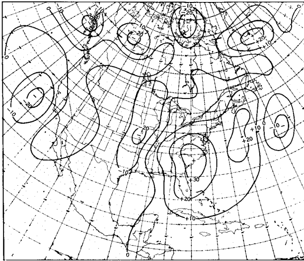
FIGURE 8.—Error in decafect of 12-hr. barotropic forecast from 1200 GMT December 6, 1959.
