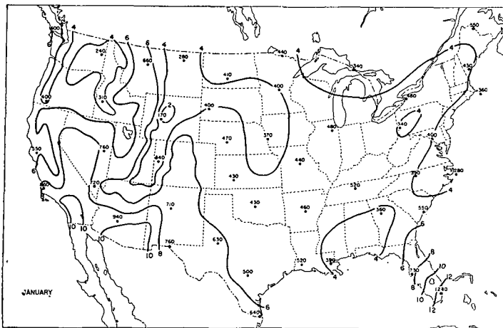
FIGURE 2.—Mean maximum mixing depths in meters above the surface during January. Isoleths are labeled in hundreds of meters.
