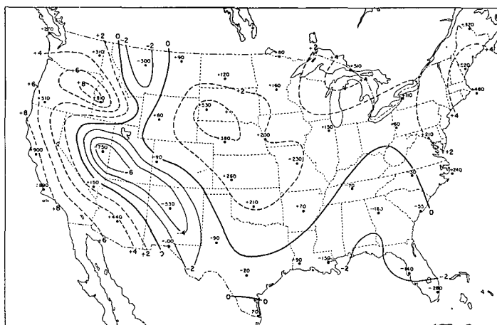
FIGURE 16.—Differences, in meters, between mean lifting condensation levels and mean maximum mixing depths during July. Negative values indicate the condensation level is less than the maximum mixing depth. Isopleths are labeled in hundreds of meters.
