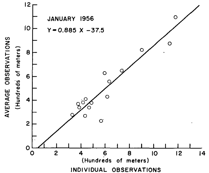
FIGURE 14.—Average maximum mixing depths during January 1956, computed from individual daily observations and from monthly average observations.
