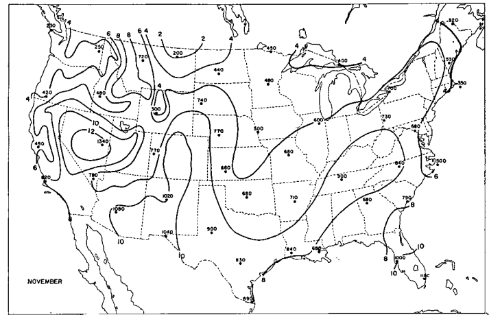
FIGURE 12.—Mean maximum mixing depths, November.
