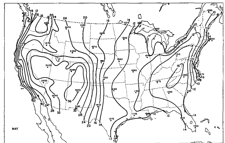
FIGURE 6.—Mean maximum mixing depths, May. Notice that over the western portion of the United States isoleths are in 400-m. intervals instead of the usual 200-m. intervals.
