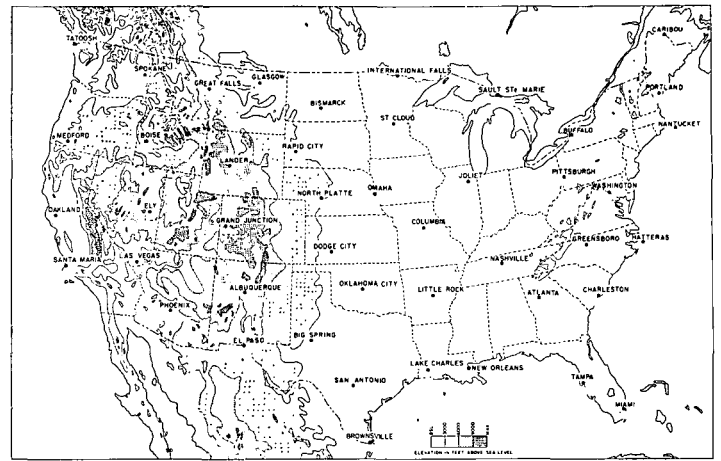
FIGURE 1.—Stations for which 10-yr. average radiosonde data are available from Ratner [2], and for which monthly mean maximum mixing depths were computed.
