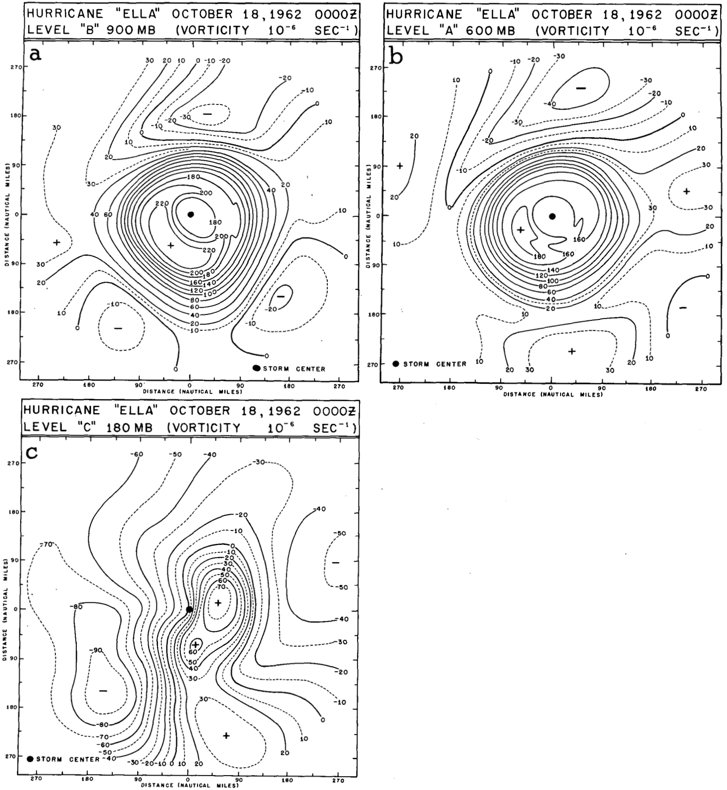
FIGURE 20.—Fields of vorticity from RFF Flights: (a) 21017-B; (b) 21017-A; (c) 21017-C.
