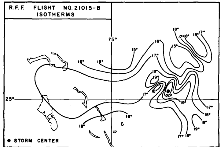
FIGURE 4.—Temperature field (°C.) from RFF observations referred to 3,240 ft., made from 1650 to 0115 GMT on October 15, 1962, by RFF Flight No. 21015–B. The analysis was made from a plot of observations at 10-min. intervals along the flight path.
