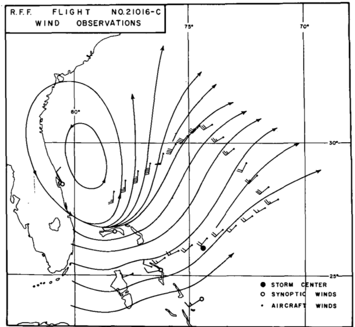
FIGURE 7.—Wind field as depicted by RFF Flight No. 21016-C (see table 1) and 43,000-ft. rawin synoptic observations at 1800 GMT, October 16, 1962.
