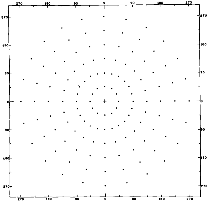
FIGURE 2.—Grid used in the computation of vorticity and divergence.
