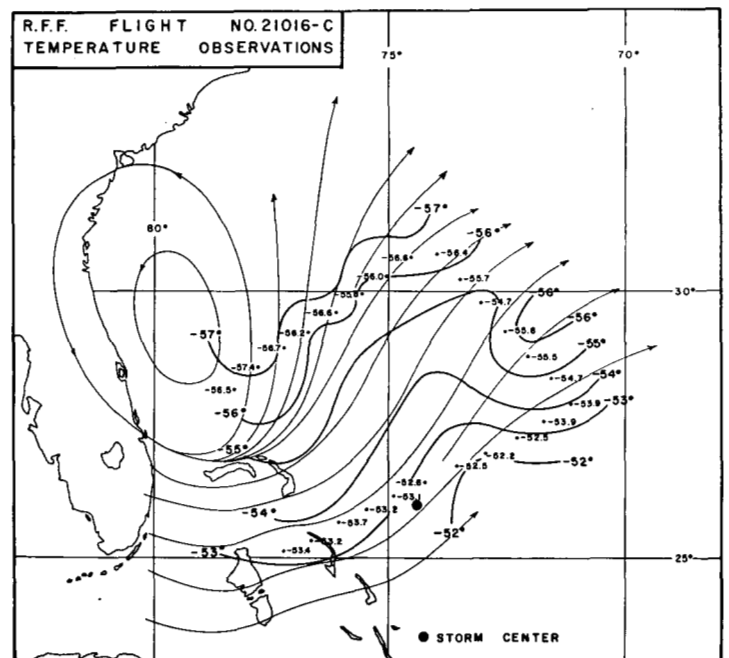
FIGURE 8.—Thick lines: isotherms (°C.) drawn from observations made by RFF Flight 21016-C (see table 1). Thin lines: streamlines reproduced from figure 7.
