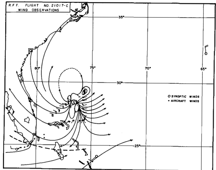
FIGURE 17.—Wind field as depicted by RFF Flight No. 21017-C (table 1) and mean layer rawins (37,000–43,000 ft.) at 0000 GMT October 18, 1962.
