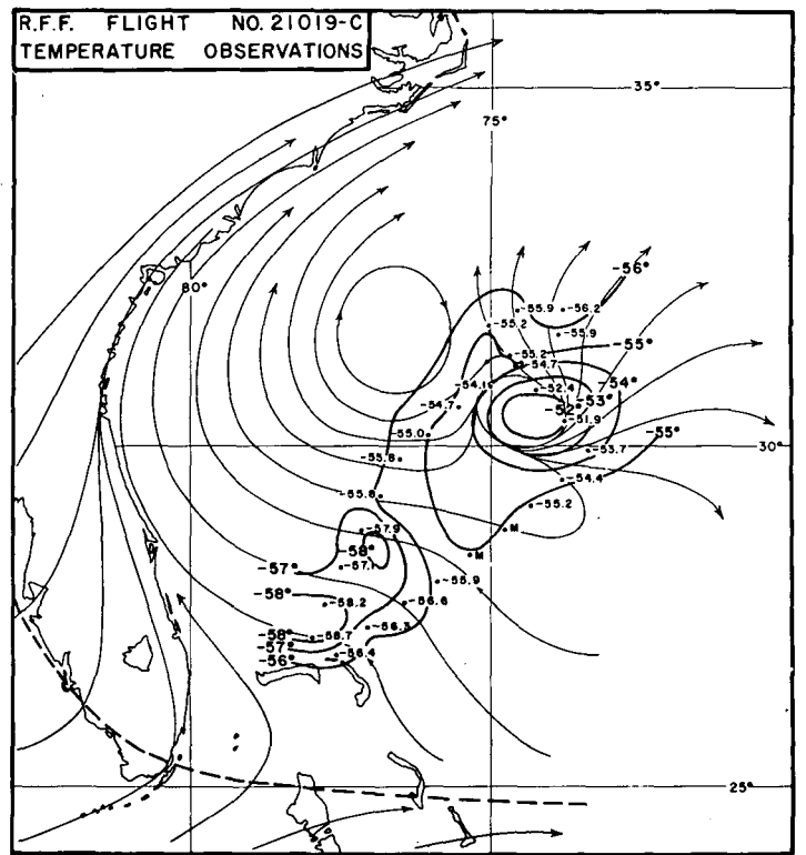
FIGURE 22.—Thick lines: Isotherms drawn from observations by RFF Flight No. 21019-C (table 1). Thin lines: Streamlines drawn from wind observations made during the same flight (not shown) and from 43,000-ft. rawin observations at 1200 GMT, October 19, 1962.
