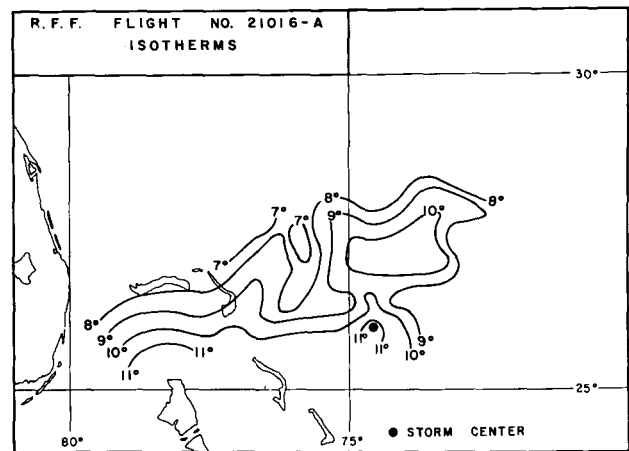
FIGURE 9.—Temperature field (°C.) from observed during RFF Flight No. 21016-A, referred to 8,090 ft.
