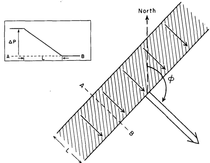
FIGURE 8.—Schematic picture of the hypothetical conditions of pressure and wind which characterize the squall line in the computations by Platzman [6, 7]. The angle φ defines the direction of motion of the squall line.
