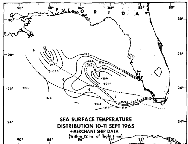
FIGURE 2.—Sea-surface temperature distribution on September 10–11, 1965.
