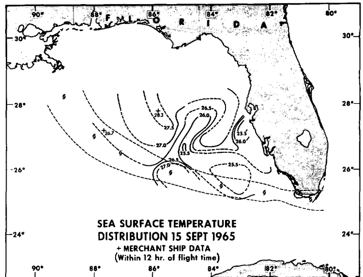
FIGURE 4.—Sea-surface temperature distribution on September 15, 1965.
