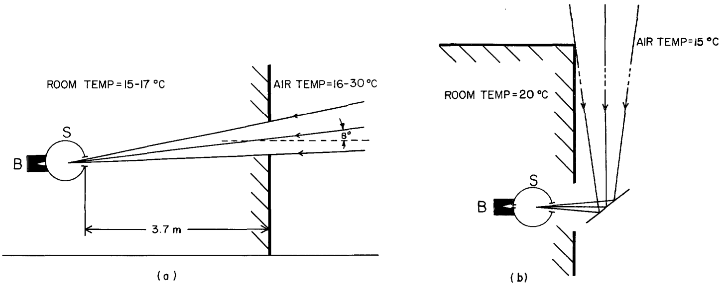
FIGURE 1.—Arrangement of the spectrometer (S) and its associated reference blackbody (B) for: (a) experiment I; and (b) experiment II. The external blackbodies used in the primary beam for calibration are not shown. The spectrometer was about 9 m. above ground level in each experiment.
