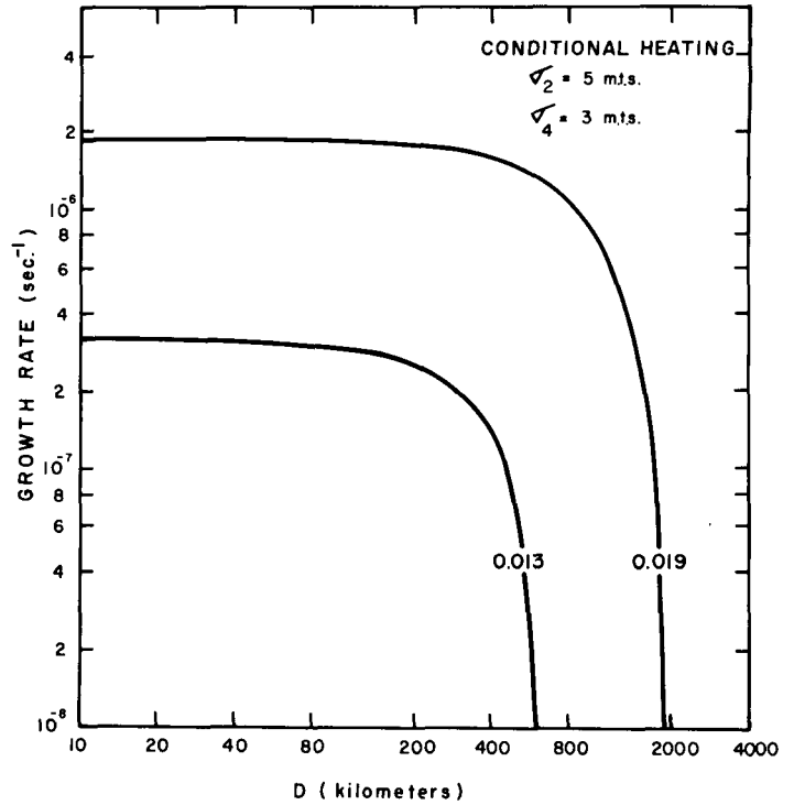
FIGURE 6.—Sample growth rate curves for conditional heating \sigma_2=5.0 m.t.s., \sigma_4=3.0 m.t.s. Curves are labeled with the appropriate values of \bar{q}_0 .
