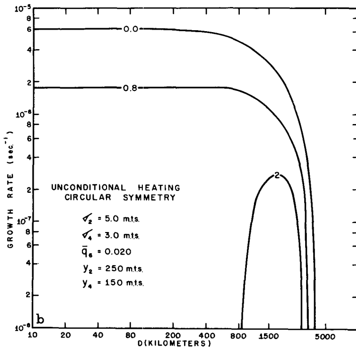
FIGURE 3.—Growth rates for unconditional heating. Curves are labeled with appropriate values of \nu . (a) \sigma_2 = 5.0 m.t.s., \sigma_4 = 3.0 m.t.s., \bar{q}_6 = .015 , (b) \sigma_2 = 5.0 m.t.s., \sigma_4 = 3.0 m.t.s., \bar{q}_6 = 0.020 .
