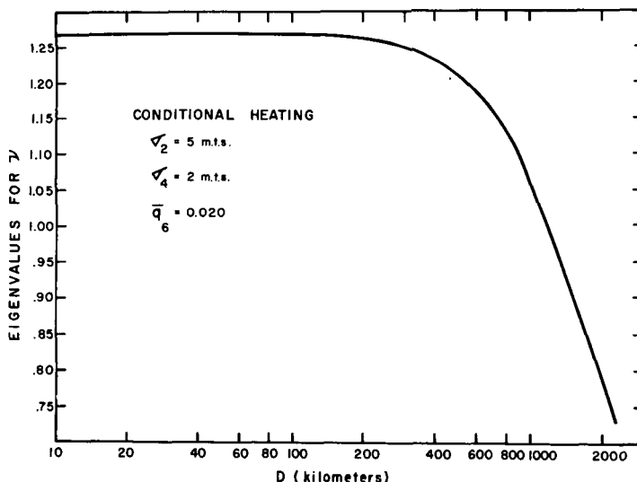
FIGURE 14.—Eigenvalues of \nu as a function of D ; \sigma_2=5.0 m.t.s., \sigma_4=2.0 m.t.s., \bar{q}_6=0.020 .
