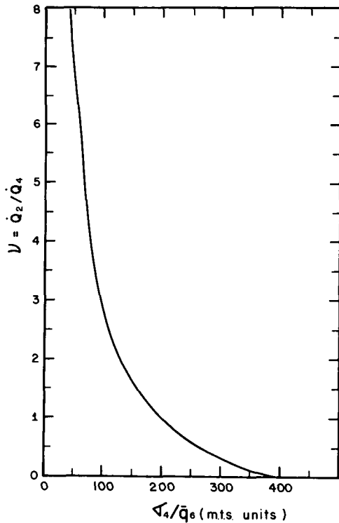
FIGURE 2.—Critical values of \nu calculated from (39). \nu measures the ratio of upper to lower tropospheric heating. When \nu exceeds the critical value, relatively small-scale disturbances are damped.
