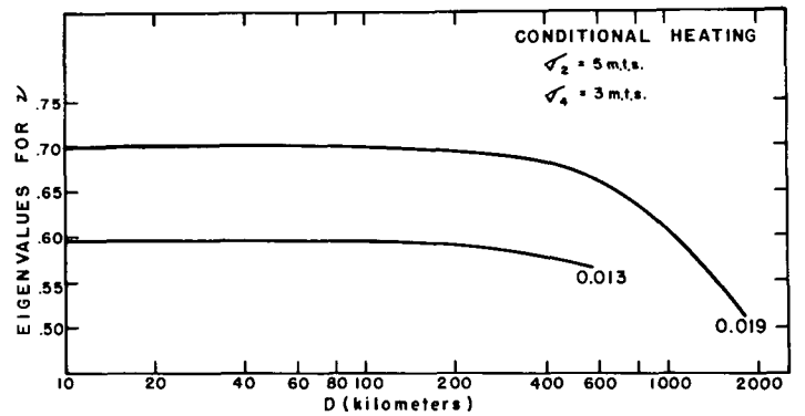
FIGURE 7.—Eigenvalues of \nu as a function of D ; \sigma_2=5.0 m.t.s., \sigma_4=3.0 m.t.s. Curves are labeled with the appropriate values of \bar{q}_0 .
