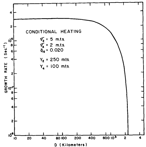
FIGURE 11.—Growth rate as a function of D ; \sigma_2=5.0 m.t.s., \sigma_4=2.0 m.t.s., \bar{q}_6=0.020 .
