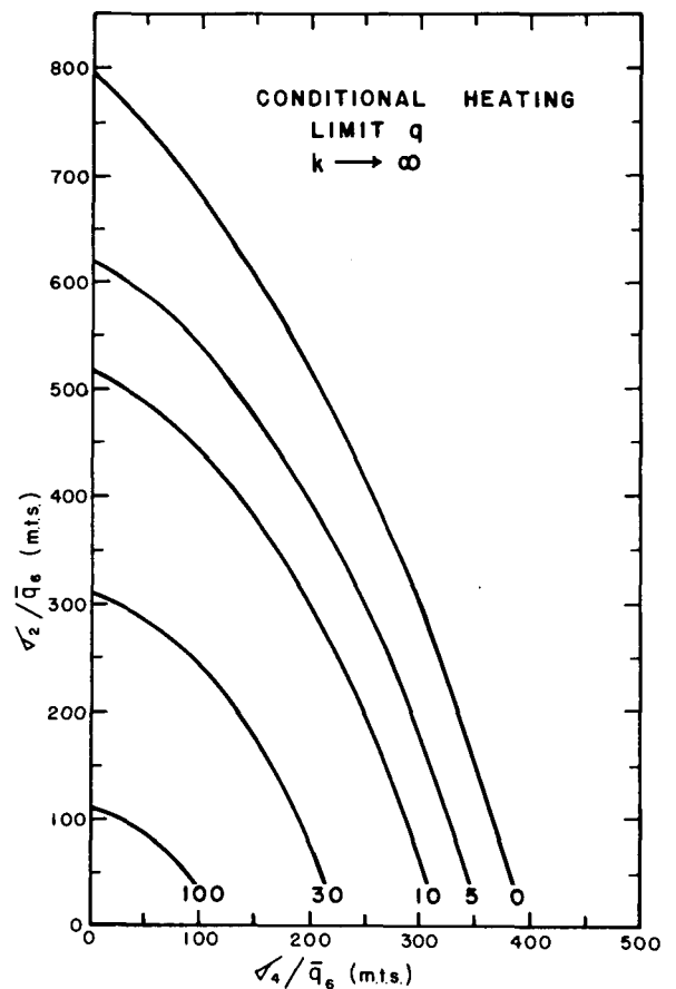
FIGURE 4.—Growth rates (conditional heating) in the limiting case as the radius of the heated region approaches zero. Isoleths are labeled in units of 10^{-7} sec. -1
