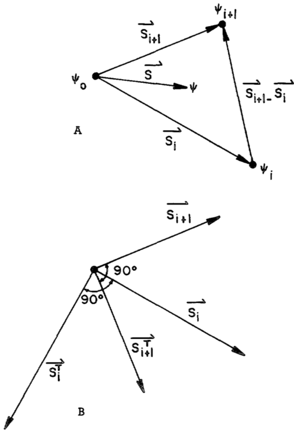
FIGURE 2.—Grid vectors.
