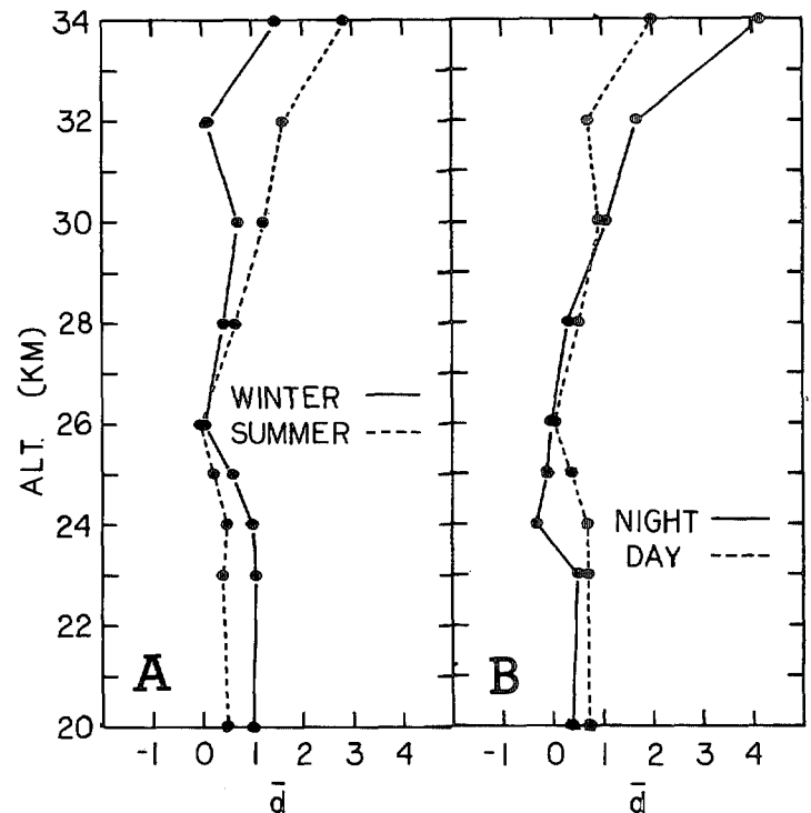
FIGURE 3.—(A) differences between the Arcasonde 1A and radiosonde mean temperatures for the winter and summer seasons. Positive values indicate colder radiosonde temperatures. (B) differences between the Arcasonde 1A and radiosonde mean temperatures for night and day. Positive values indicate colder radiosonde temperatures.
