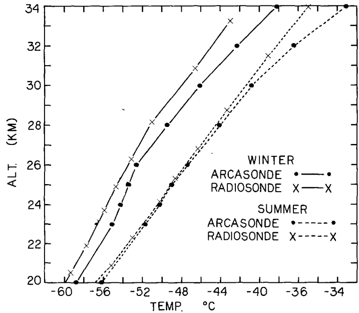
FIGURE 5.—Profiles of the 6-yr mean rocketsonde temperatures and 3-yr mean radiosonde temperatures for Wallops Island, Va.
