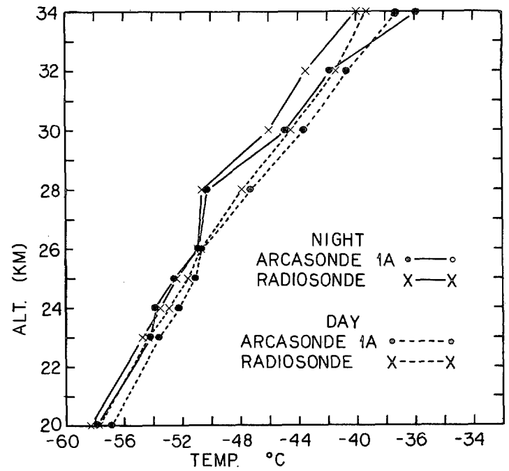
FIGURE 2.—Arcasonde 1A and radiosonde mean-temperature profiles for all night and day data at Wallops Island, Va.
