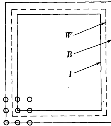
FIGURE 1.—Rectangular 47×51 grid point network. The dashed line W represents the solid walls in the fluid. The full line B represents the boundary of the grid, and I represents the first set of interior points.
