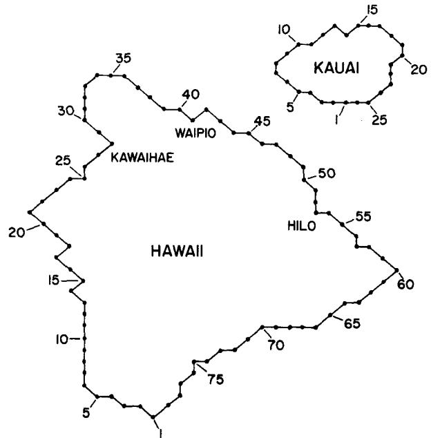
FIG. 6. Key for grid points around the model islands of Kauai and Hawaii.
