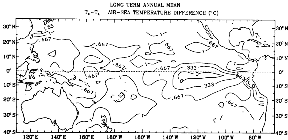
FIG. 12. Annual mean sea surface minus surface air temperature difference (°C) for 1957-76.
