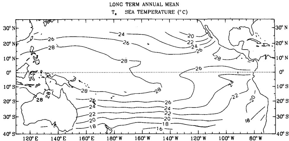
FIG. 2. Annual mean sea surface temperature ( ^{\circ}\text{C} ) for the period 1957–76. Values are based upon 5^{\circ} \times 5^{\circ} grid averages of the marine data described in the text.
