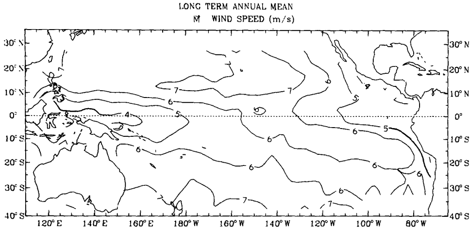
FIG. 8. Annual mean wind speed ( \text{m s}^{-1} ) for 1957-76.
