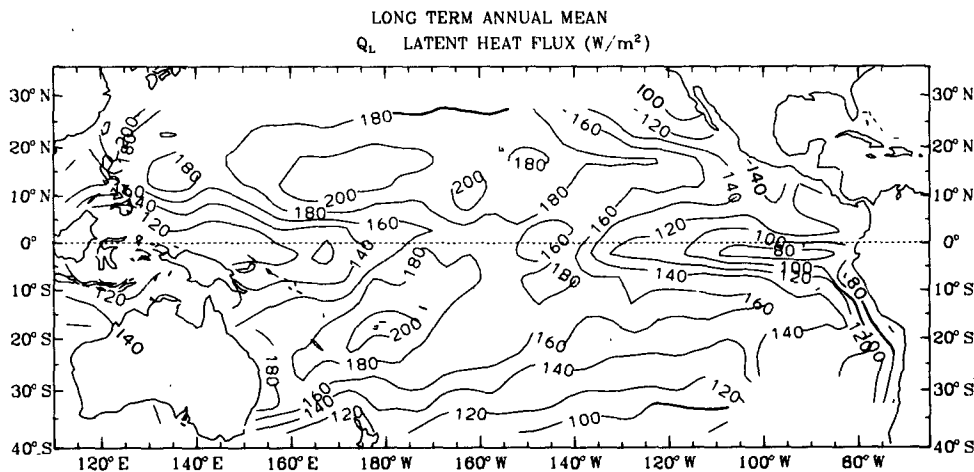
FIG. 7. Annual mean loss of latent heat through evaporation ( W m^{-2} ) for 1957-76.
