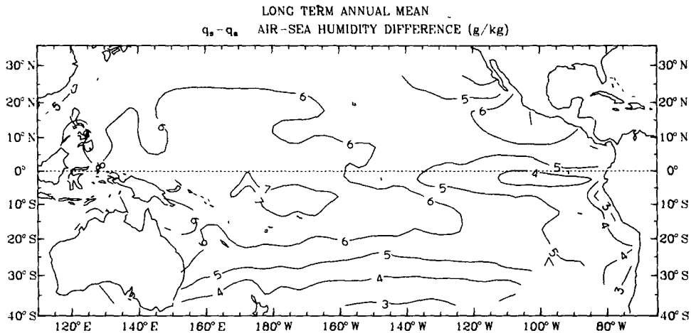
FIG. 9. Annual mean humidity difference ( \text{g kg}^{-1} ) for 1957-76.
