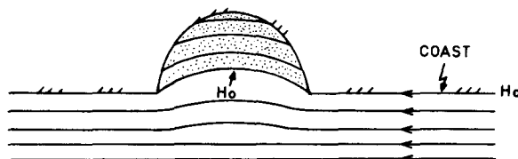
FIG. 2. Topographically induced blockage. Flow approaches from right. Solid lines imply the isobaths.
