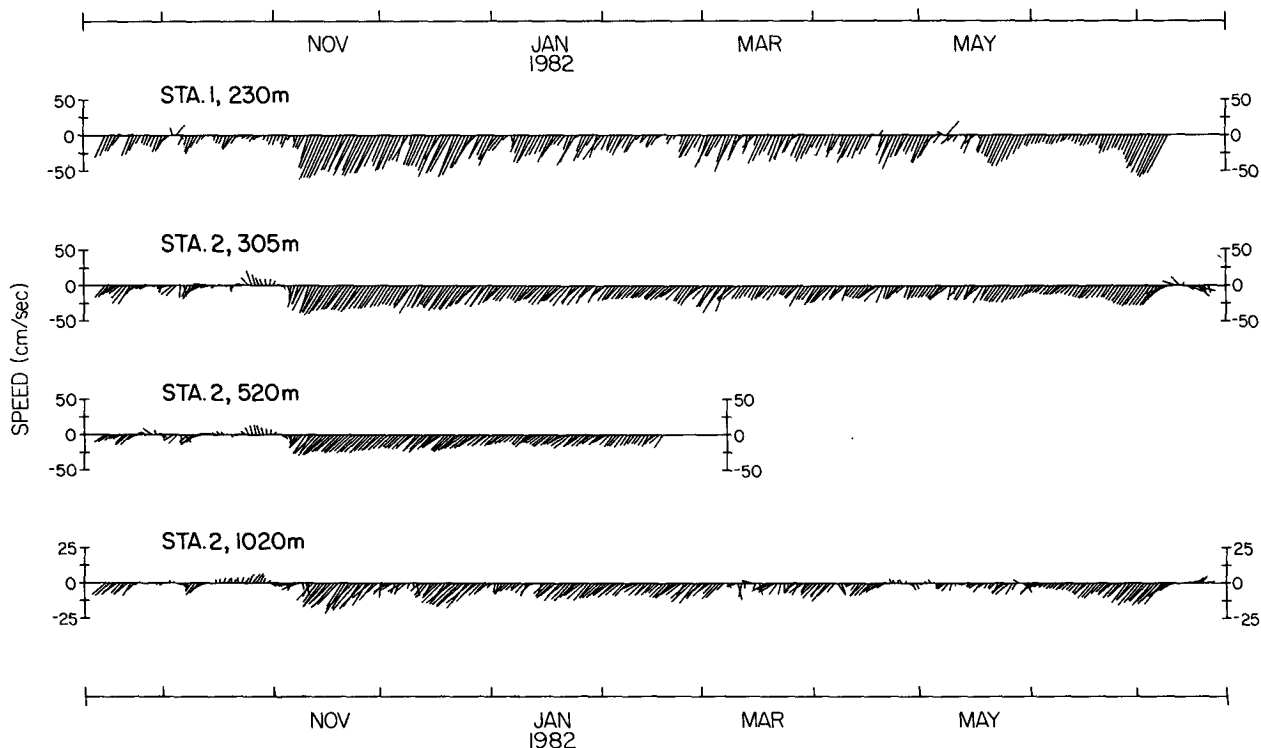
FIG. 2. Daily net current vectors (after use of a 35-hour filter) at stations 1 and 2, 15 September 1981-21 July 1982. North is up on these plots.
