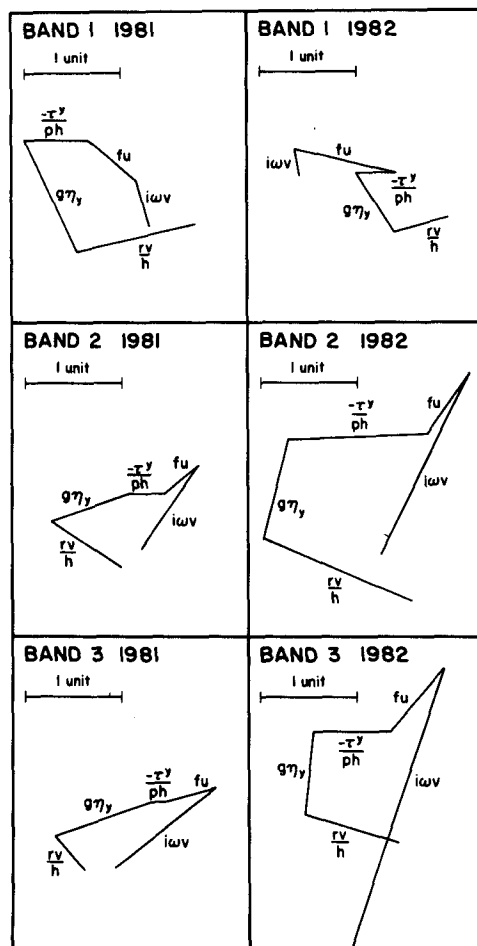
Fig. 9. As in Fig. 8 but alongshore.
