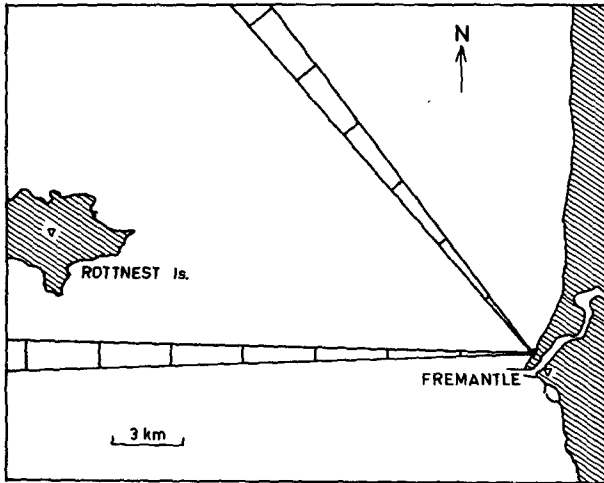
FIG. 2. The experiment site showing the two selected beam azimuths. The assumption is made that the wind and wave fields are independent of longshore displacement and functions of offshore dimension. Fremantle is located at 31°03'S, 115°44'E.
