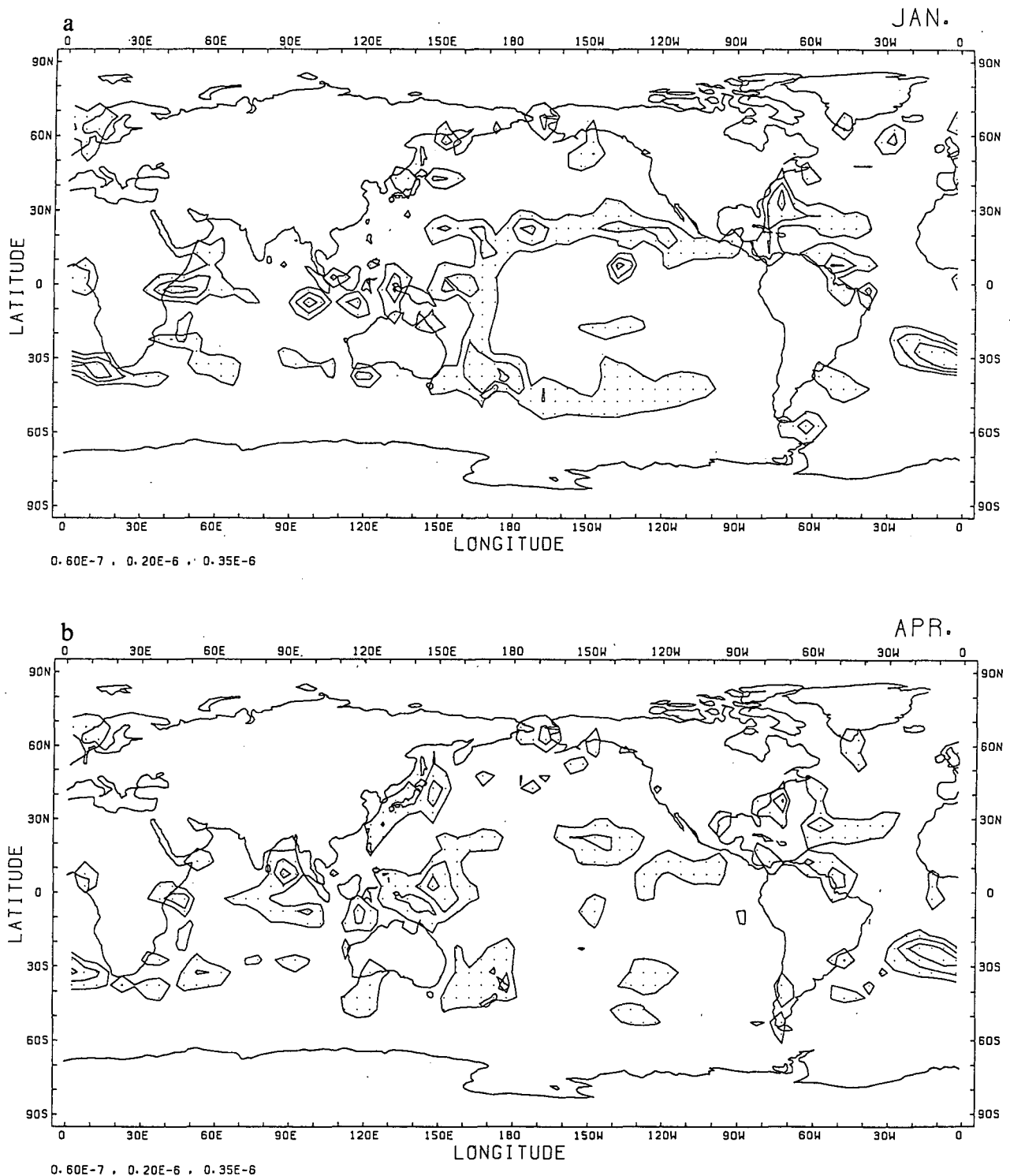
FIG. 6. Convergence fields for each season. (a) January, (b) April, (c) July, (d) October. The contour lines are 0.60 \times 10^{-7} s^{-1} , 0.20 \times 10^{-6} s^{-1} and 0.35 \times 10^{-6} s^{-1} .
