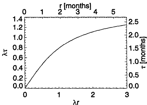
FIG. 1. Normalized time lag \lambda\tau of standard restoring boundary conditions as a function of normalized restoring time \lambda r . Also shown are the time lag \tau (mo) as a function of restoring time r (mo) for the particular case of the annual cycle.
