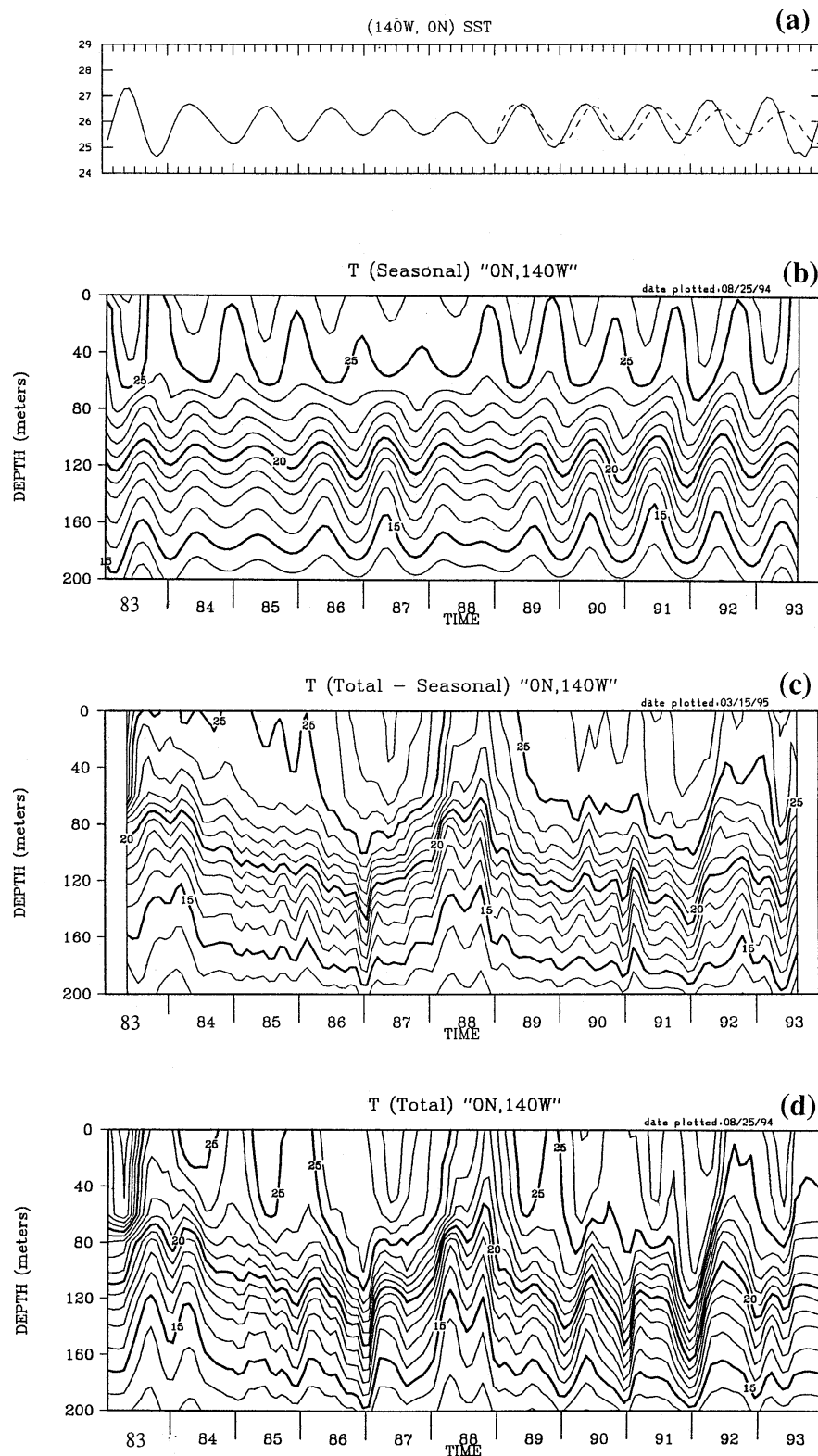
FIG. 7. Same as Fig. 7 but for 0^{\circ} , 140^{\circ}\text{W} .
