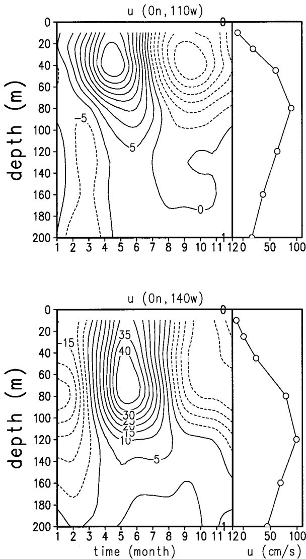
FIG. 3. The mean (on the right of the panel) and seasonal variations (on the left of the panel) of zonal currents at 110^{\circ}\text{W} (upper panel) and 140^{\circ}\text{W} (lower panel) with contour interval 5\text{ cm s}^{-1} . Negative values indicate westward flow.
