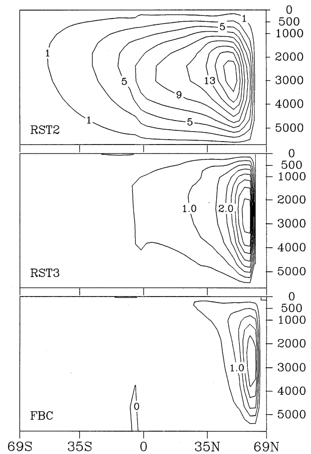
FIG. 9. EOF1 of meridional overturning for RST2 (top, contour interval 2 Sv), RST3 (middle, contour interval 0.5 Sv), FBC (bottom, contour interval 0.5 Sv).
