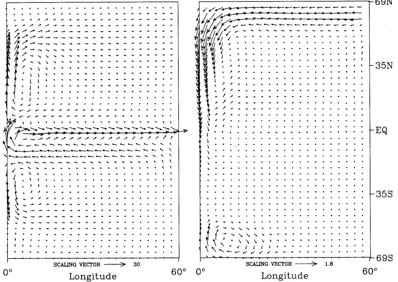
FIG. 3. Meridional section of density at 20° longitude (in sigma units, top left), meridional streamfunction (in Sv, top right), and horizontal velocity fields (in \text{cm s}^{-1} ) at level 2 (bottom left) and level 13 (bottom right) for the pole-to-pole equilibrium state used as initial condition for the stochastically forced experiments.
