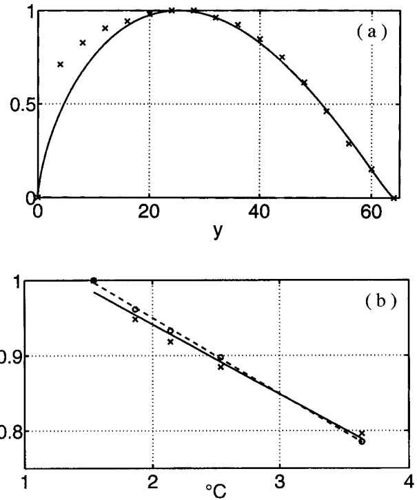
FIG. 12. (a) Latitudinal dependence of northward heat transport according to the scaling [ Eq. (13), solid] and from the numerical experiment (see Fig. 1a; boundary mixing case, k_v = 5 \times 10^{-4} \text{ m}^2 \text{ s}^{-1} ; crosses). (b) Maximum heat transport from the numerical runs divided by meridional overturning at 32^\circ\text{N} , plotted against horizontally averaged bottom temperature from the model. Overturning at 32^\circ\text{N} is taken either from the scaling [Eq. (17); crosses, solid line] or the model solution (circles, dashed line). Both sets of heat transport to overturning ratios have been normalized by their respective maximum values. The lines are least squares fits.
