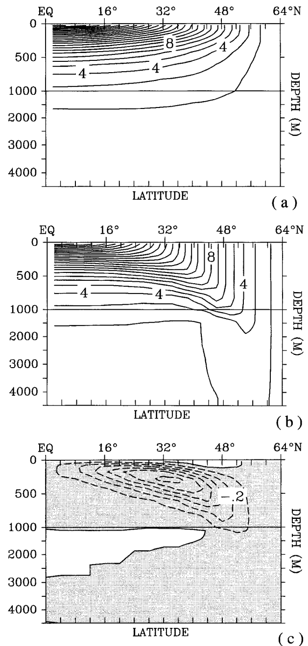
FIG. 4. Boundary mixing case, k_v = 5 \times 10^{-4} \text{ m}^2 \text{ s}^{-1} . (a) Temperature along the western boundary, contour interval 1°C. (b) Temperature along the eastern boundary, contour interval 1°C. (c) Potential density difference as eastern wall minus western wall, contour interval 0.1 kg m -3 . Areas with negative values are marked by dashed contours and shading.
